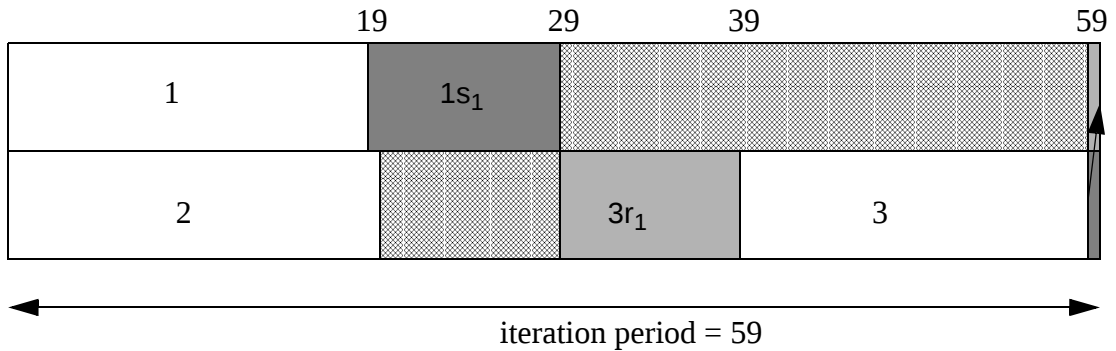
Figure 7. Gantt Chart for ST schedule with \text{exec}(1)=19 .
