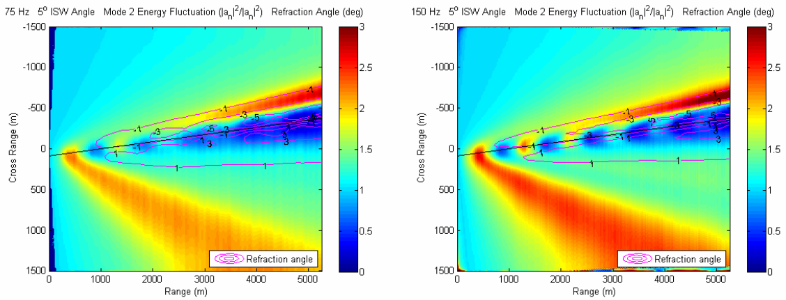
Figure 14. Normal mode energy fluctuation, |A_n|^2 / |A_{n0}|^2 , for ISW angle of 5^\circ and mode 2, overlaid with the refraction angle in degrees. The 75 Hz case is shown in the left panel and 150 Hz on the right.
