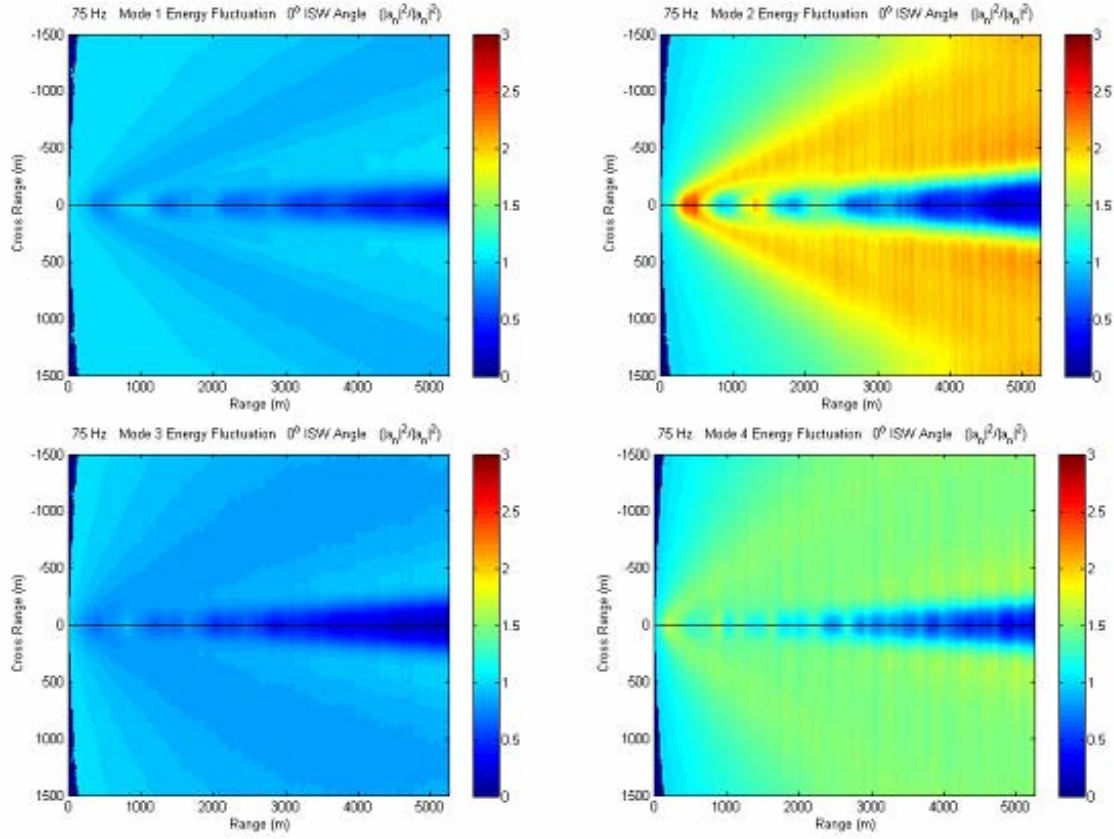
Figure 4. Normal mode energy fluctuation, |A_n|^2 / |A_{n0}|^2 , at 75 Hz for ISW angle of 0^\circ and modes 1-4. Mode 1 is shown in the upper left panel, mode 2 upper right, mode 3 lower left, and mode 4 lower right.
