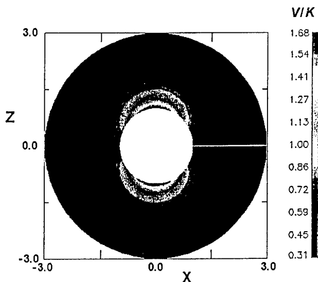
Fig. 10. Normalized potentials for the case R=1.0 , \alpha=1.2 , \phi_b=23.9 , Y=0 .
