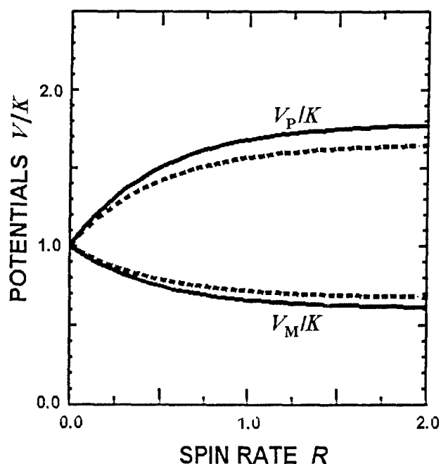
Fig. 4. The average normalized bellyband potential, V_M/K , and the average spin pole potential, V_P/K , versus R . The dashed lines indicate the threshold values.
