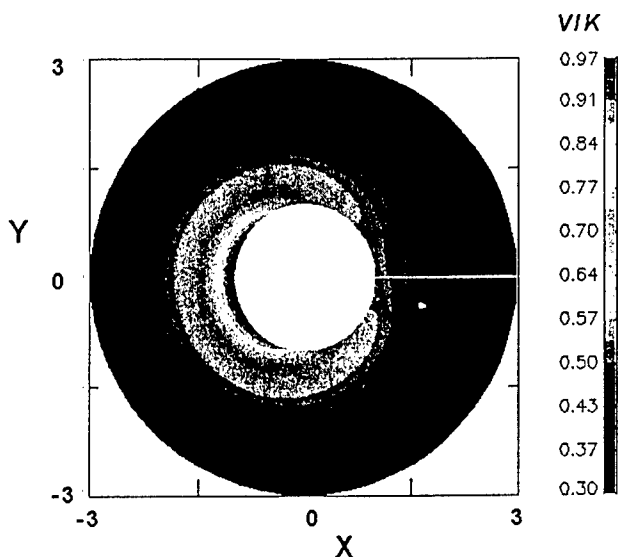
Fig. 11. Normalized potentials for the case R=0.5 , \alpha=1.2 , \phi_b=9.3 , Z=0 .
