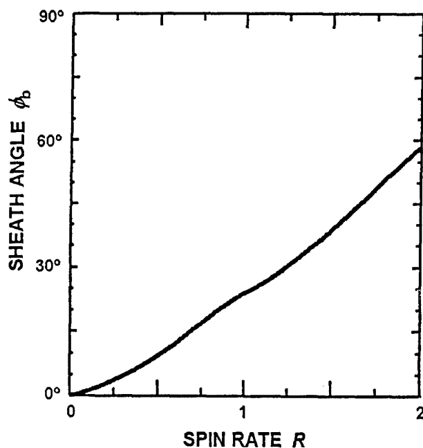
Fig. 5. The photoemission sheath angle, \phi_b , at the maximum sheath radius, versus R .
