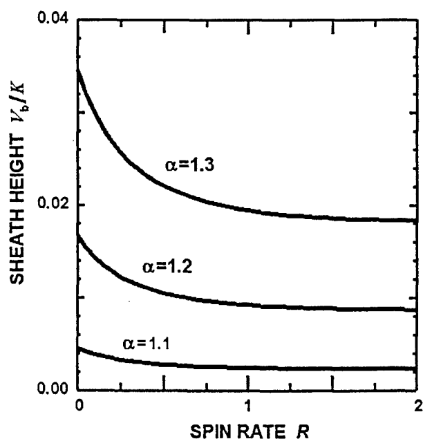
Fig. 7. The normalized photoemission sheath barrier height, V_b/K , at \phi_b , versus R .
