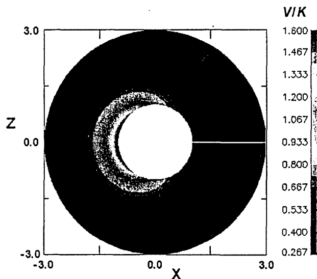
Fig. 8. Normalized potentials for the case R = 0.0 , \alpha=1.2 , \phi_b=0 , Y=0 .
