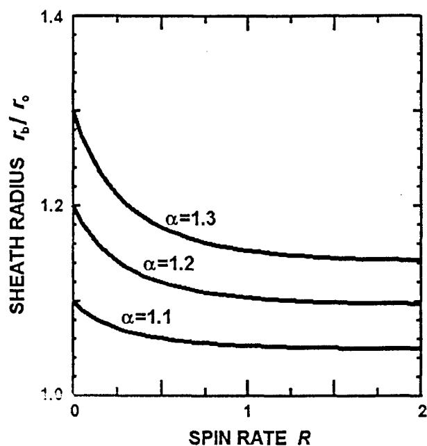
Fig. 6. The photoemission sheath radius, r_b , at \phi_b , versus R .
