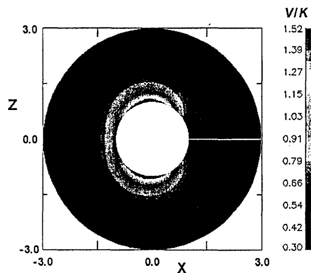
Fig. 9. Normalized potentials for the case R=0.5 , \alpha=1.2 , \phi_b=9.3 , Y=0 .
