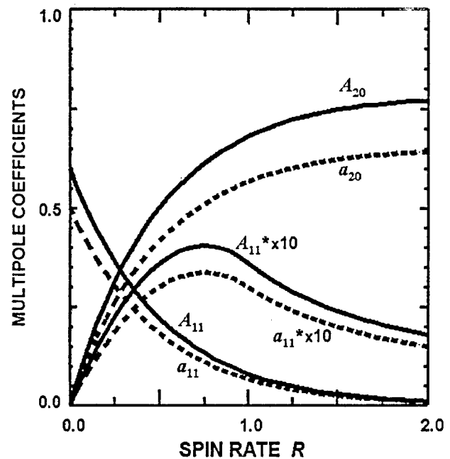
Fig. 3. Representative plots showing the R dependence of the absolute value of the multipole coefficients. The solid lines are for \alpha=1.2 and the dashed lines for \alpha=1.0 . The A_{11}^* terms are multiplied by 10 for clarity. The differential charging voltages, D and d , are obtained by multiplying A_{11} and A_{11}^* by -2K .
