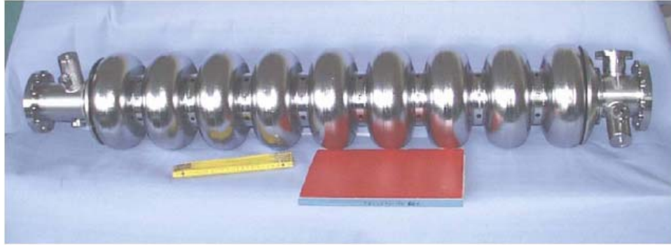
Figure 3. An example of a RF accelerator ([From Ref. [5].])
