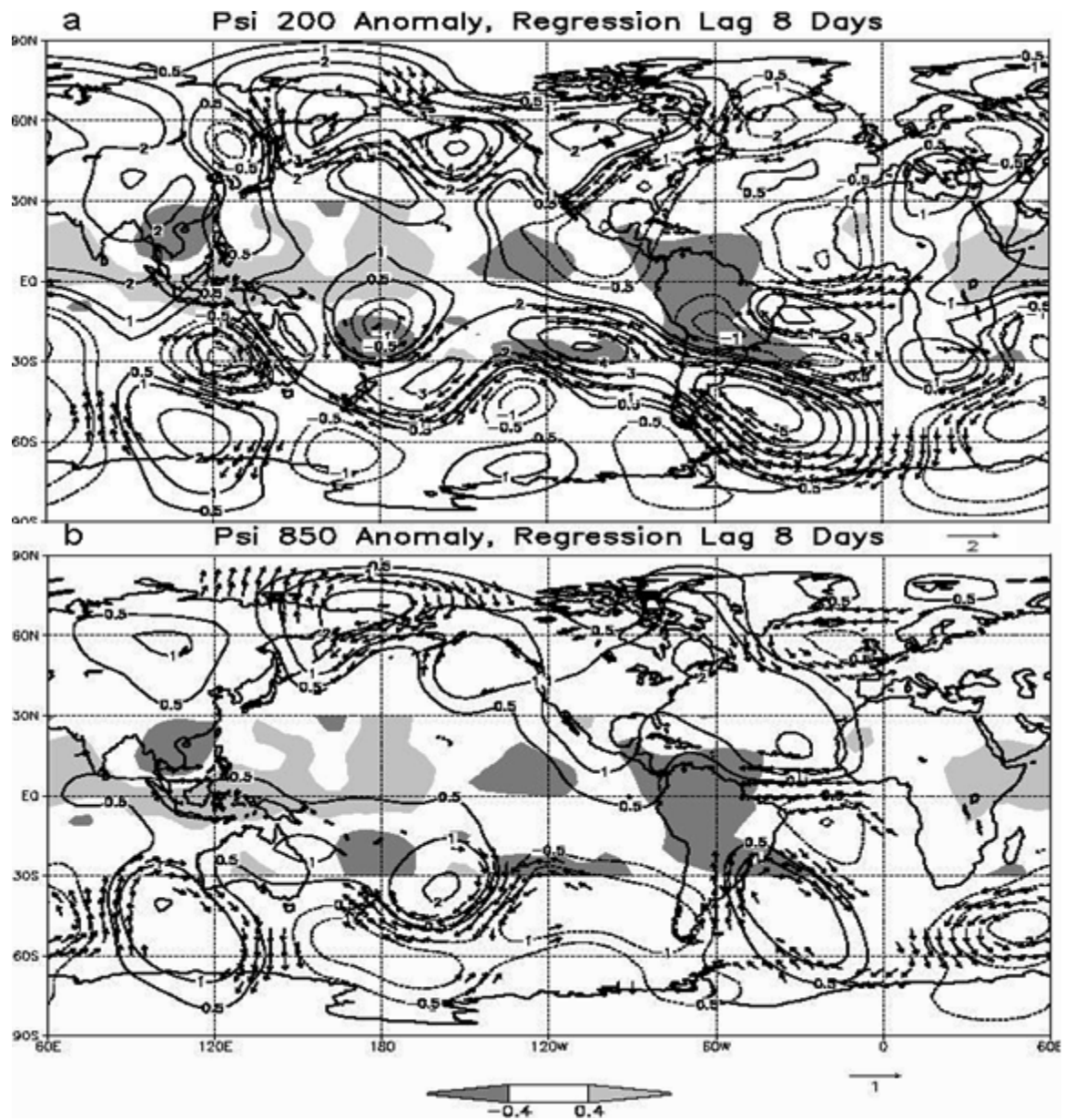
Figure 3.14 As in Figure 3.6, except for lag +8 days.
