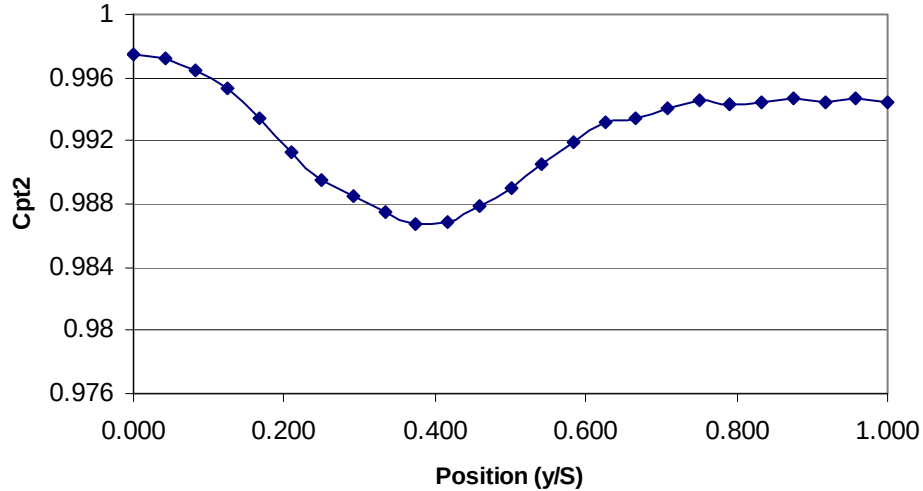
Figure 12. Non-dimensional pressure distribution in the blade wake at midspan
