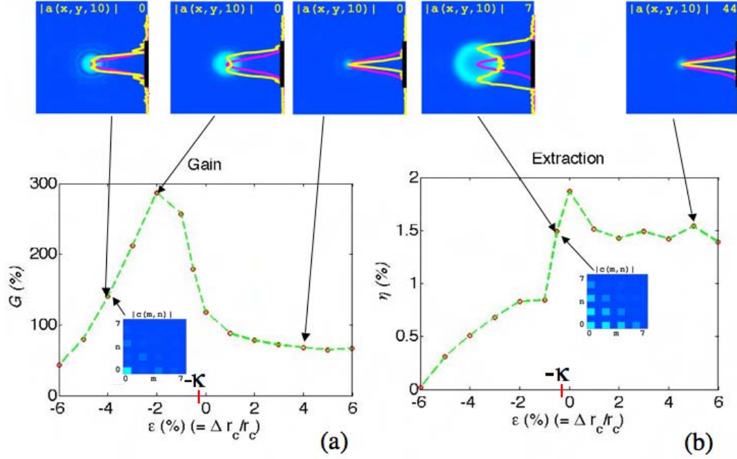
Figure 29. (a) Gain trend for spherical distortion for the JLab STI wiggler. (b) Extraction trend for spherical distortion for the JLab STI wiggler
