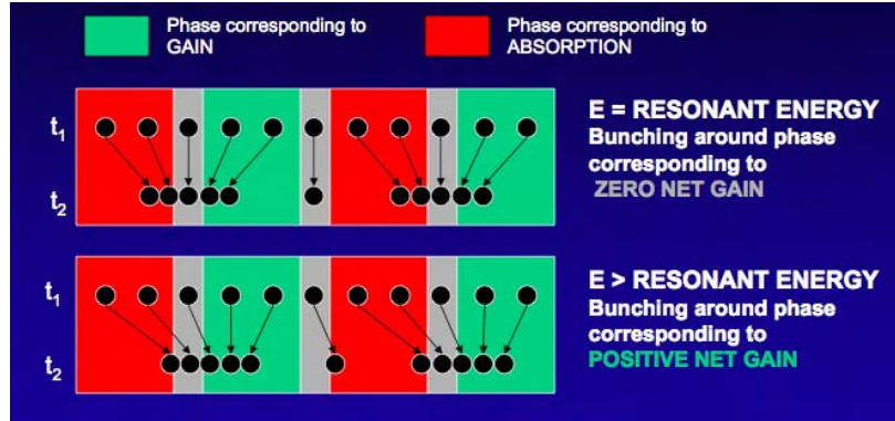
Figure 11. In the upper picture, electrons have an initial \nu_o = 0 which results in bunching but no gain. In the lower picture, electrons have an initial \nu_o > 0 resulting in good bunching and positive gain from [4].
