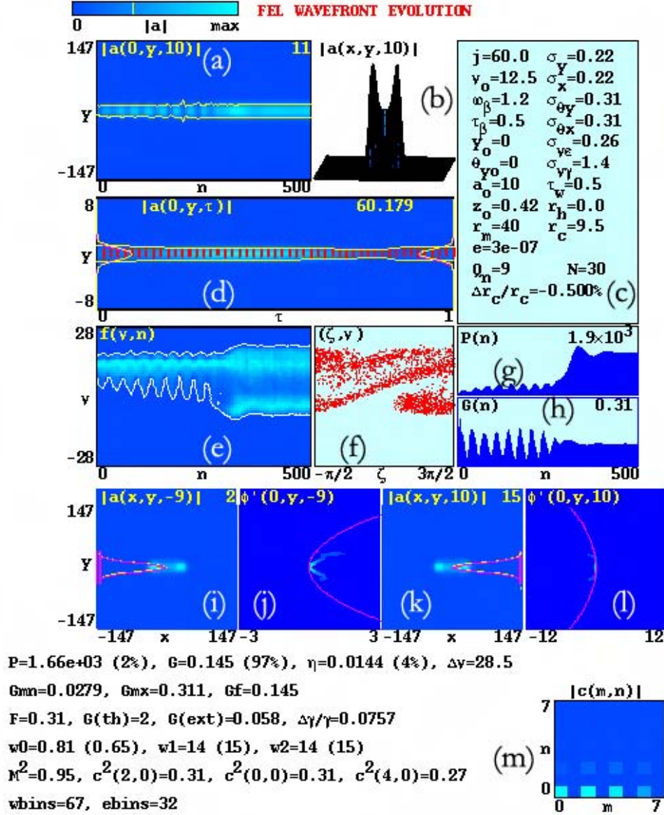
Figure 21. FEL simulation output. (a) Optical mode evolution over 500 passes at right mirror (b) Surface plot of the optical field at the right mirror after last pass; (c) User defined parameters (see Table (III)); (d) Cross section of optical mode and electron beam as it propagates from \tau = 0 \rightarrow 1 on last pass; (e) Evolution of electron beam distribution in phase velocity over 500 passes; (f) Electron phase space at \tau = 1 after last pass; (g) Optical power evolution over 500 passes; (h) Optical gain evolution over 500 passes; (i) Burn pattern of optical mode at left mirror after last pass; (j) Optical phase for at left mirror after last pass; (k) Burn pattern of optical mode at right mirror after last pass; (l) Optical phase for at right mirror for last pass; (m) Hermite-Gaussian coefficients for right mirror (Code is developed in this chapter)
