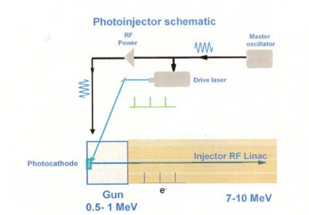
Figure 4. Schematic of a typical photoinjector from [6].
