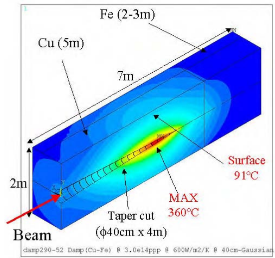
Figure 7. Beam dump from [9]
