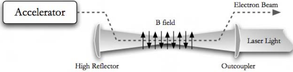
Figure 2. Free electron laser system in an oscillator configuration from [5].
