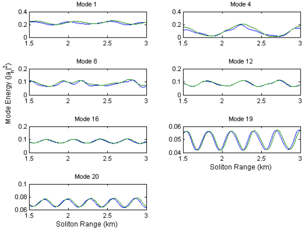
Figure 25. Comparison of simulated (blue) and theoretical (green) results for the seven highest energy modes of a 300-Hz sound source at 60m, and a single wave moving between 1.5 and 3km. The similarity in both the mode pattern and mode energy is surprising at this relatively high frequency.
