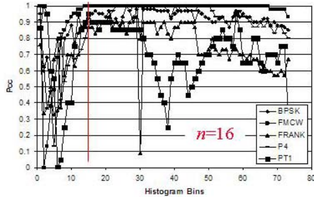
Figure 48. Choi-Williams Optimization Table (Test Noise).
