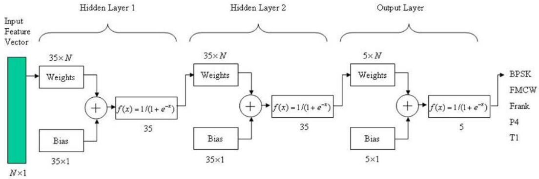
Figure 30. Three-layer Perceptron Used for Classification.
