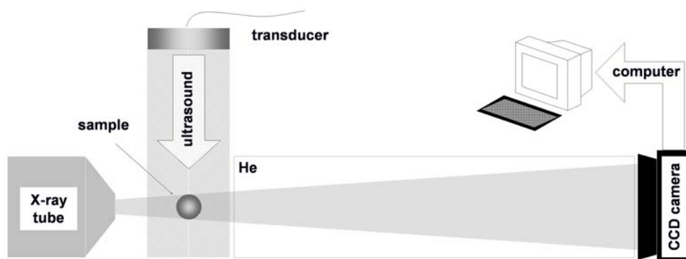
Figure 1 : Diagram of the experimental apparatus. X-radiation generated by a microfocus tube penetrates a sample and is detected by a CCD camera that views a scintillation plate. The CCD camera is read by the computer which stores the images and performs the subtractions.
