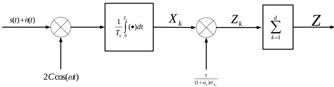
Figure 19. The modified noise-normalized combining receiver.
