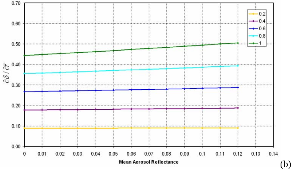
Figure 7. The change in AOD with a change of 100% in mean aerosol reflectance as a function of mean aerosol reflectance for a solar zenith angle of (a) 0° and (b) 30°, for a sensor zenith angle 0° and surface reflectance curves for values ranging from 0.2 to 1.0.
