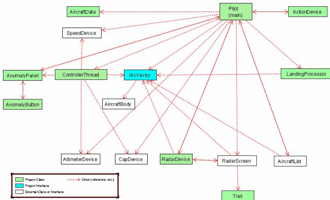
Figure 27. The UML diagram of the cockpit module
