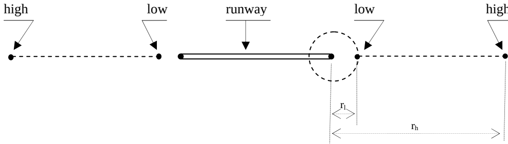
Figure 36. Runway extensions
