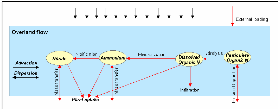
Figure 5. Overland flow nitrogen transport and transformation module.
