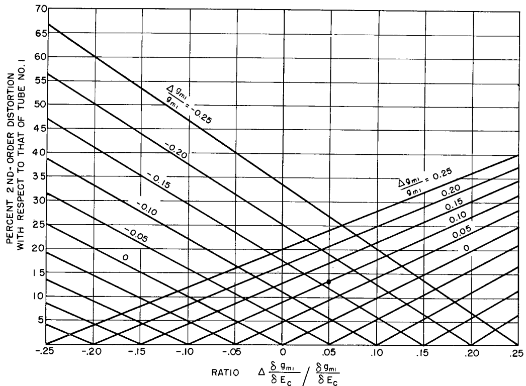
Fig. 3 - Percent second-order distortion in push-pull amplifier relative to that of single tube as a function of difference in tube characteristics
