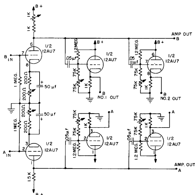
Fig. A1 - Circuit diagram of experimental push-pull multicoupler
