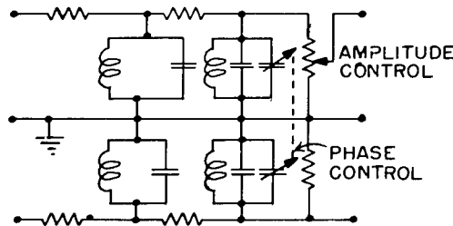
Fig. A3 - Typical filter used in measuring circuit
