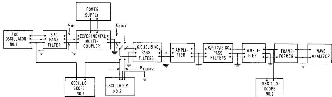
Fig. A2 - Block diagram of distortion-measuring system used with experimental push-pull multicoupler
