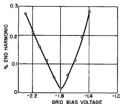
Fig. 6 - Percent second harmonic as a function of the grid bias of the output cathode follower
