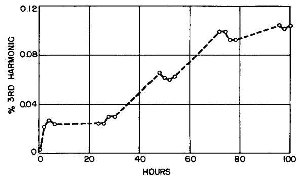
Fig. 12 - Variation of the percent third harmonic of multicoupler with time in the 100-hour stability test
