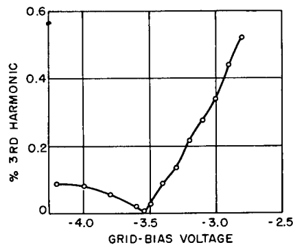
Fig. 11 - Percent third harmonic as a function of the grid bias of the output cathode follower
