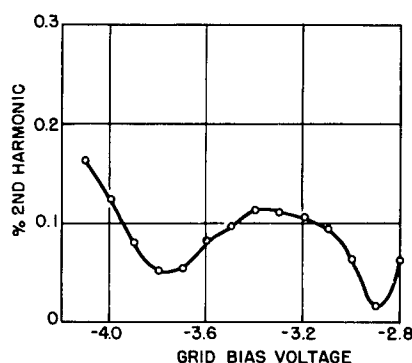
Fig. 5 - Percent second harmonic as a function of grid bias of the input amplifier
