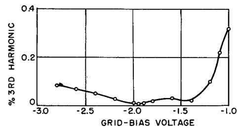
Fig. 10 - Percent third harmonic as a function of the grid bias of the input amplifier
