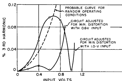
Fig. 8 - Percent third harmonic as a function of the multicoupler input-signal amplitude with the circuit adjusted for third-harmonic cancellation
