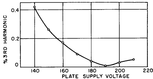
Fig. 9 - Percent third harmonic as a function of the multicoupler plate-supply voltage
