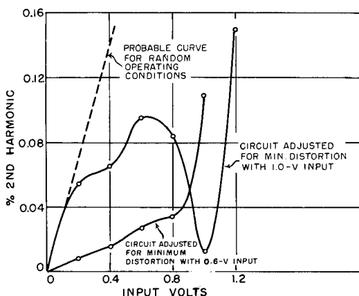
Fig. 7 - Percent second harmonic as a function of the multicoupler input-signal amplitude with the circuit adjusted for second-harmonic cancellation
