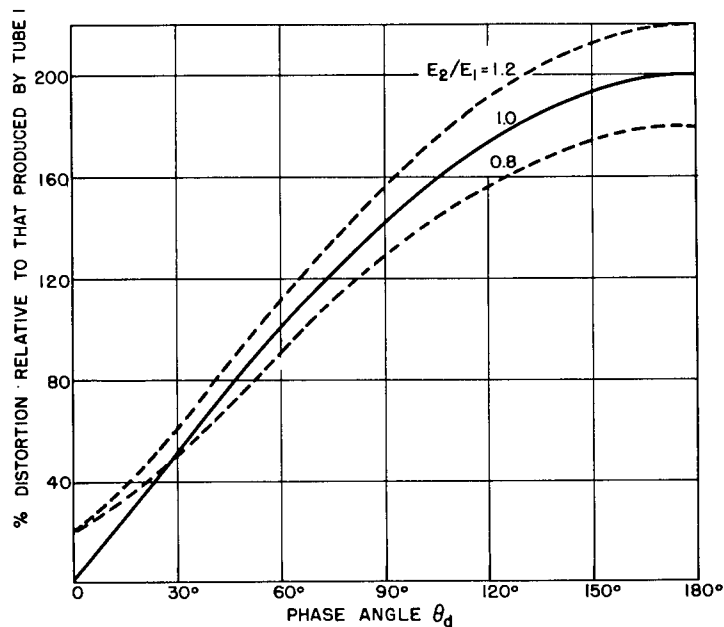
Fig. 2 - Percent even-order distortion in push-pull amplifier relative to that of single tube as a function of amplitude and phase difference
