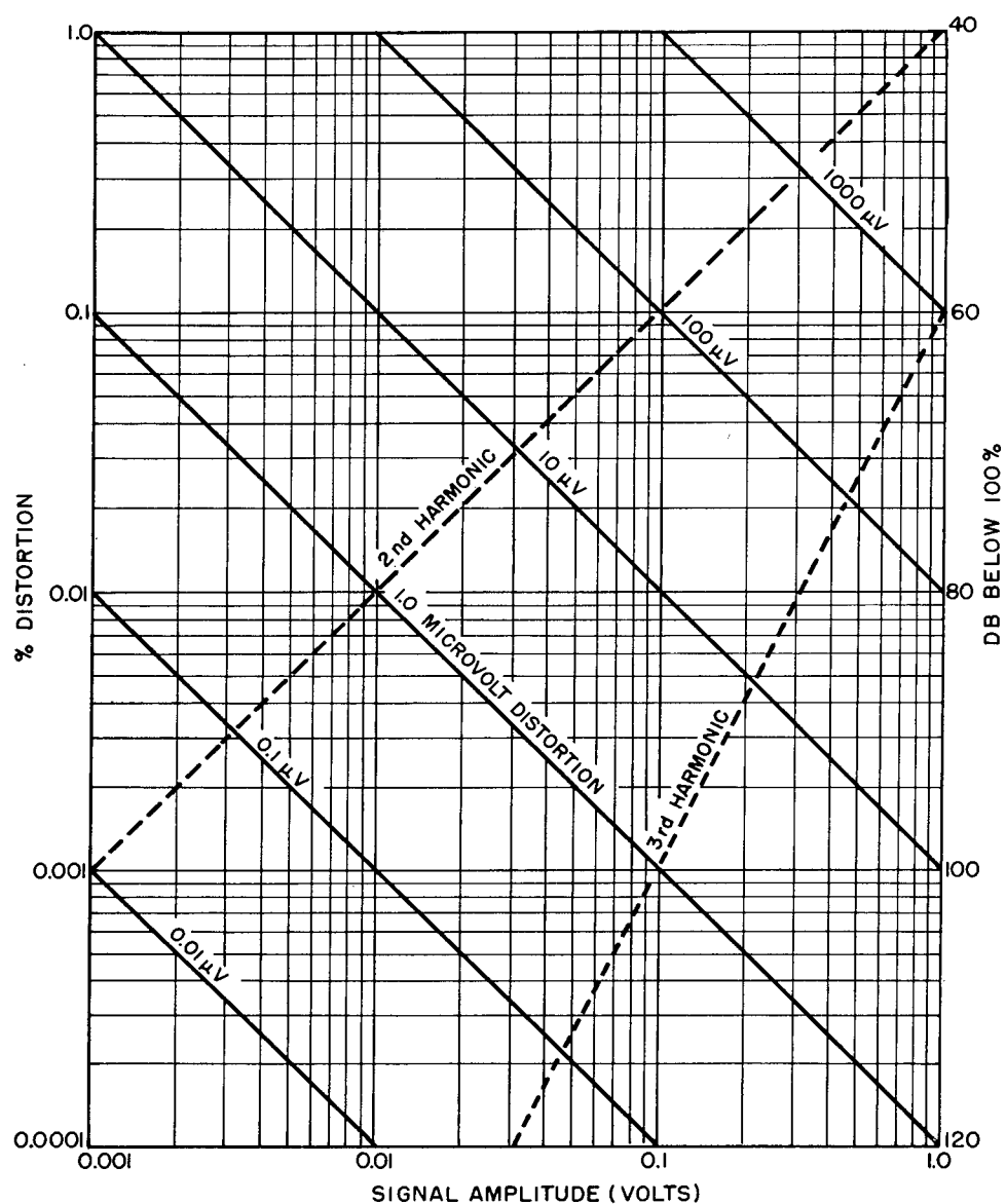
Fig. 1 - Distortion voltage as a function of signal amplitude and percent distortion
