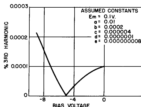
Fig. 4 - Percent third harmonic as a function of grid bias for assumed tube constants
