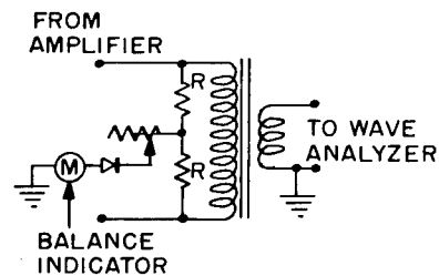
Fig. A4 - Transformer and balance indicator
