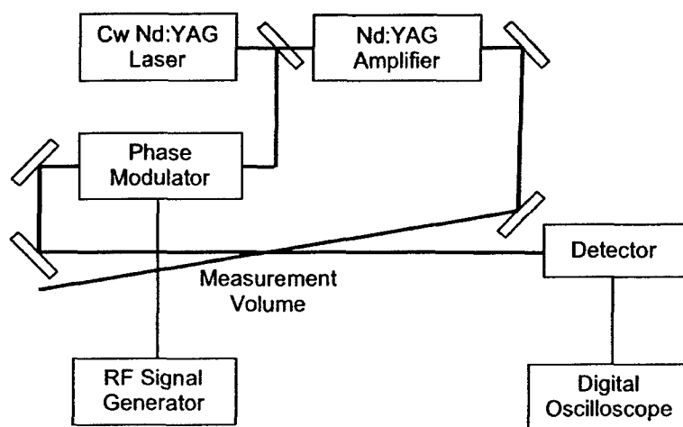
Figure 10. Schematic of pulsed stimulated scattering measurement with FM detection.
