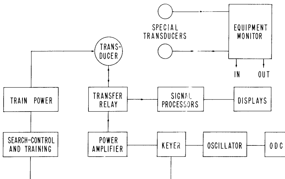
Figure 4 - Major components
