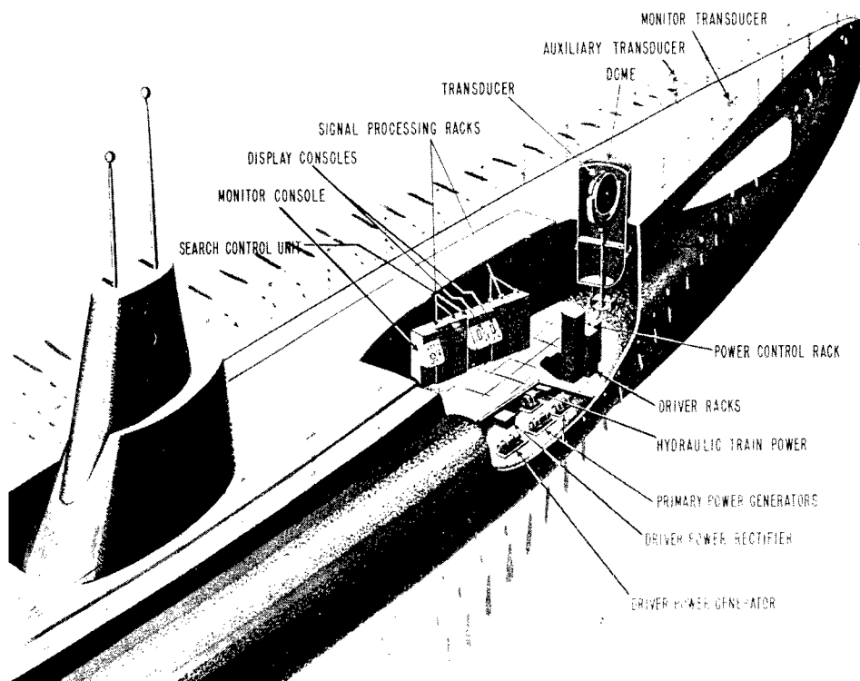
Figure 3 - Location of components in forward torpedo room of U.S.S. GUAVINA
