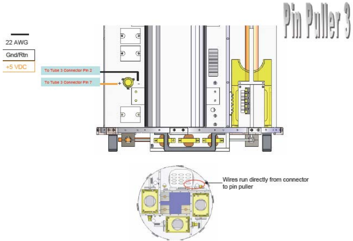
Figure E-8: Pin Puller 3
