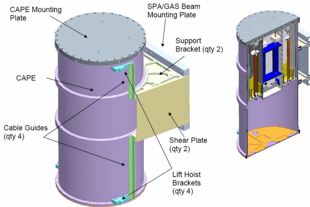
Figure 3.3.1: CAPE/RIGEX Assembly
