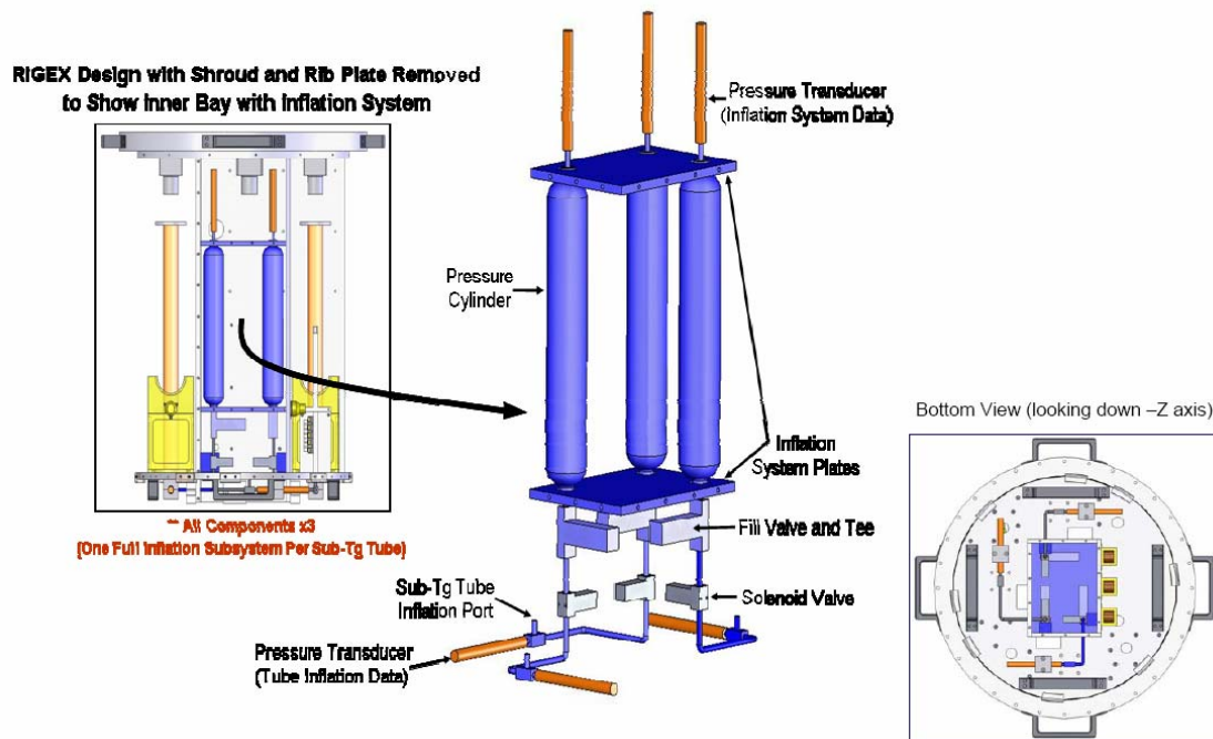
Figure 3.1.5c: RIGEX Inflation System
