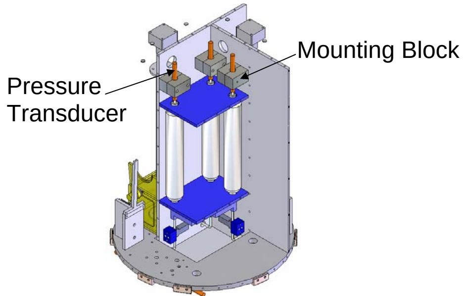
Figure 5.4-1: Three Pressure Transducers for Nitrogen Gas Tanks
