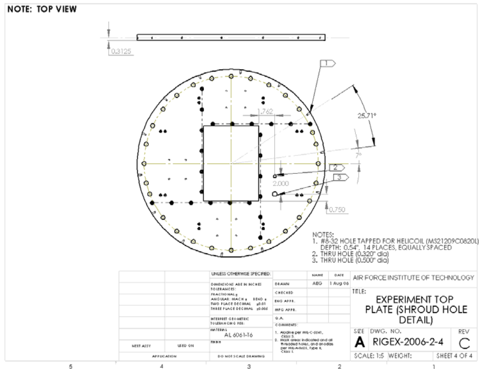
Figure D-7: Experiment Top Plate View 4
