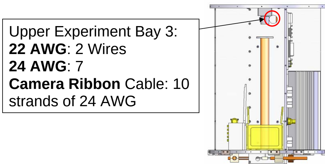
Figure E-20: Experiment Bay 3 Wire Routing Totals
