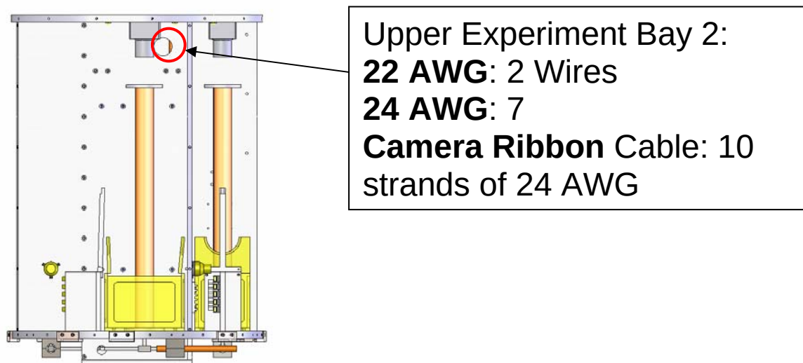
Figure E-19: Experiment Bay 2 Wire Routing Totals
