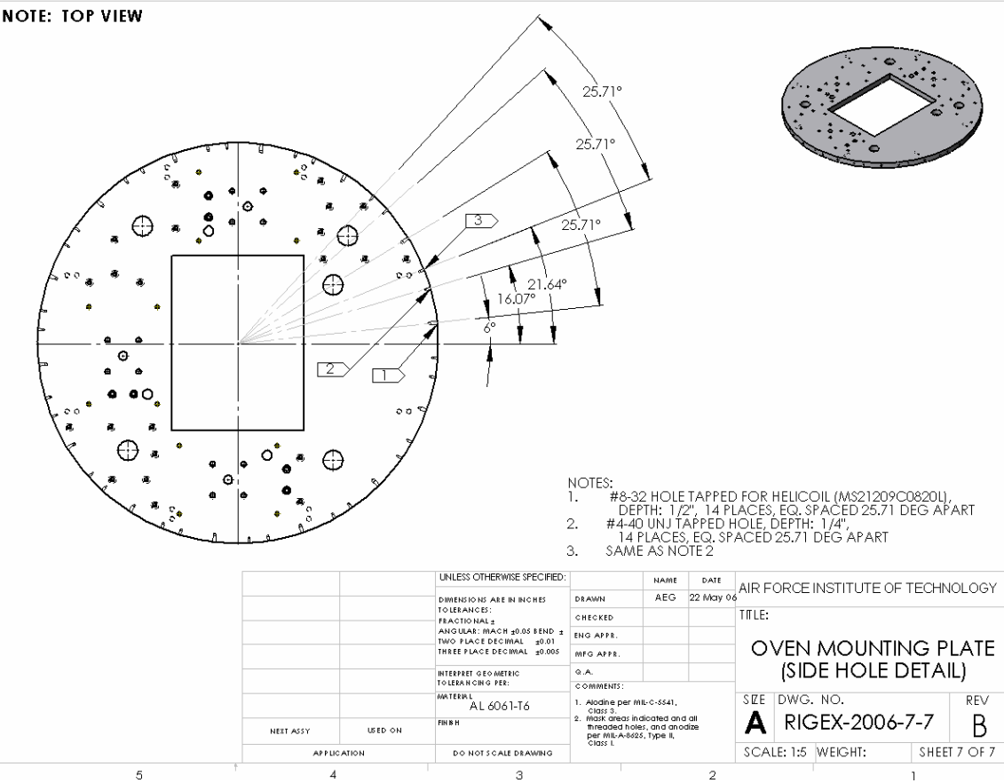
Figure D-23: Oven Mounting Plate View 7
