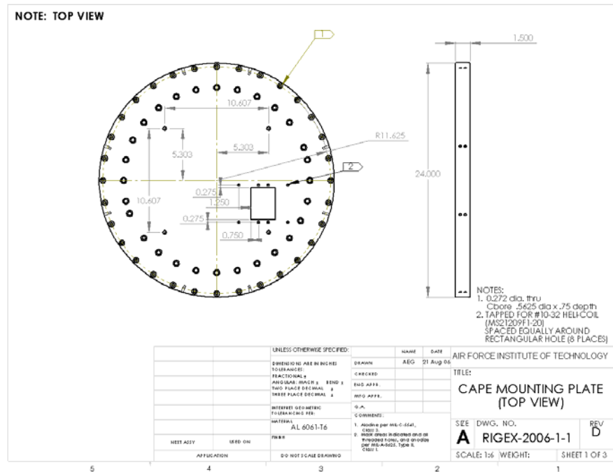
Figure D-1: CAPE Mounting Plate View 1
