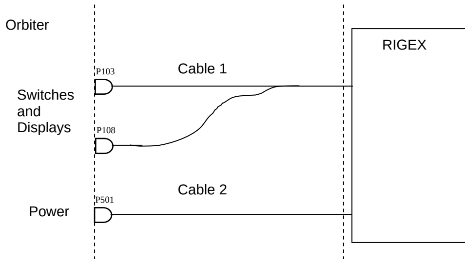
Figure 5.7-1: RIGEX/Orbiter Interface Cable Routing
