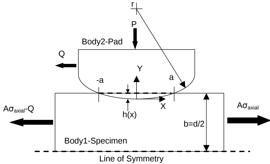
Figure 2.3. Free body diagram of fretting fatigue loads.
