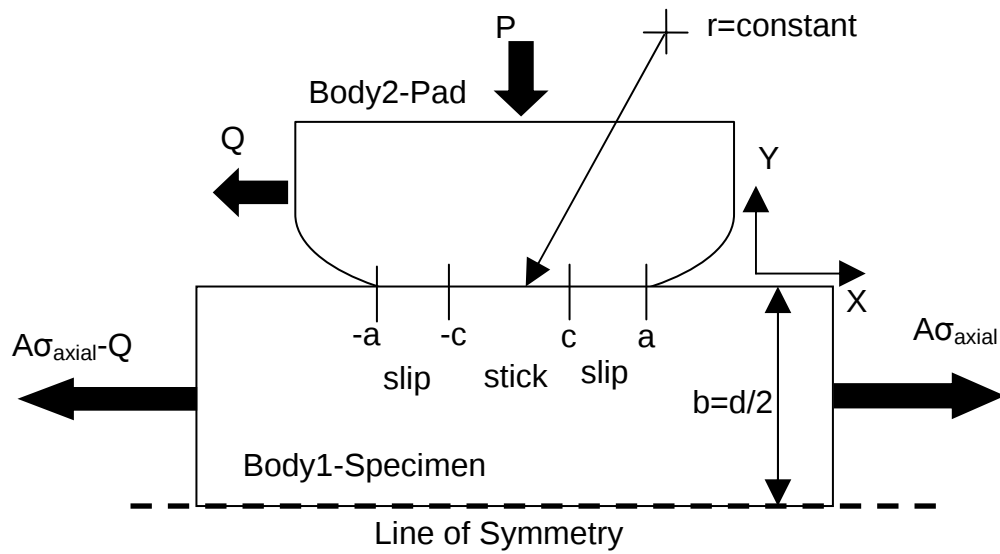
Figure 2.4. Partial slip conditions in fretting fatigue configuration.
