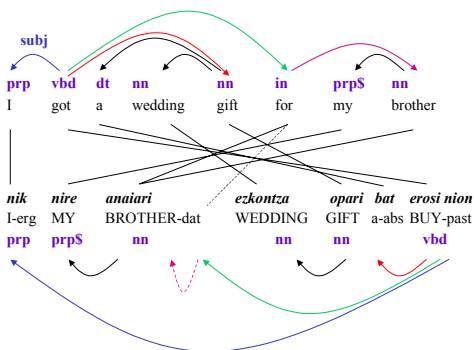
Figure 2. An example of dependency transfer
