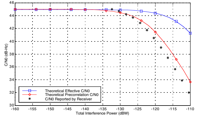
Figure 12. Results for Band-Edge Interference, Theory Uses Receiver Front-End Bandwidth 16 MHz, Model B Receiver
