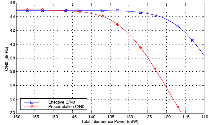
Figure 5. Theoretical Results for Narrowband Interference Offset from Band Center by 7.5 Times the Chip Rate, Receiver Front-End Bandwidth 16 MHz
