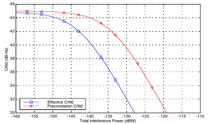
Figure 1. Theoretical Results for Narrowband Interference at Band Center, Receiver Front-End Bandwidth 8 MHz
