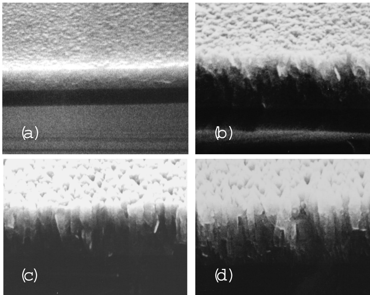
Fig. 8. The SEM micrographs of SiC-thin films grown on Si 3 N 4 /Si structures with 30 sccm 3MS and 1 sccm N 2 at the following temperatures: (a) 1100°C, (b) 1150°C, (c) 1200°C, and (d) 1250°C.
