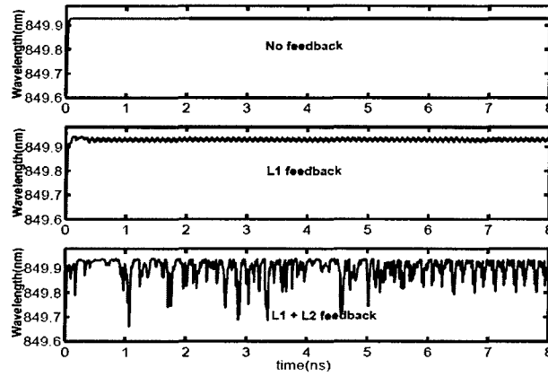
Fig. 25. Effect of optical feedback on output wavelength in a single lens and two lens system.
