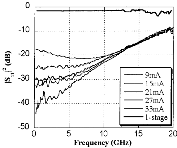
Figure 3.15. 3-stage S11-parameters.
