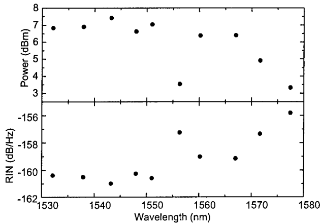
Figure 3.5. Fiber-coupled optical power and the corresponding RIN values at 0.2 GHz, of ten optimized channels along the >45 nm tuning range.
