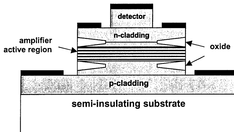
Figure 4.4. Schematic showing the design of the GaAs-based TAP detector
