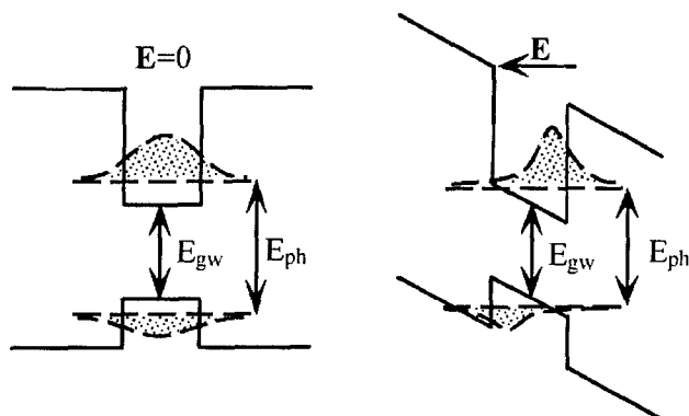
Figure 1.1. Quantum confined Stark effect.
