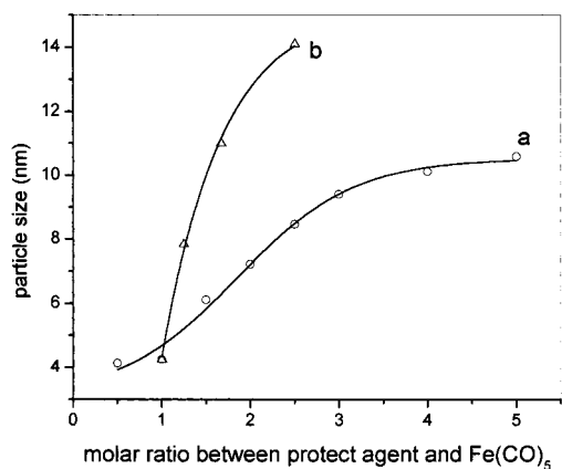
Figure 7. Effect of the molar ratio between protective agent and Fe(CO) 5 . (a) The initial amount of Fe(CO) 5 was fixed at 1.00 mmol, and the amount of protective agent varied. (b) The amount of protective agent was fixed at 1.00 mmol and the amount of Fe(CO) 5 was changed.
