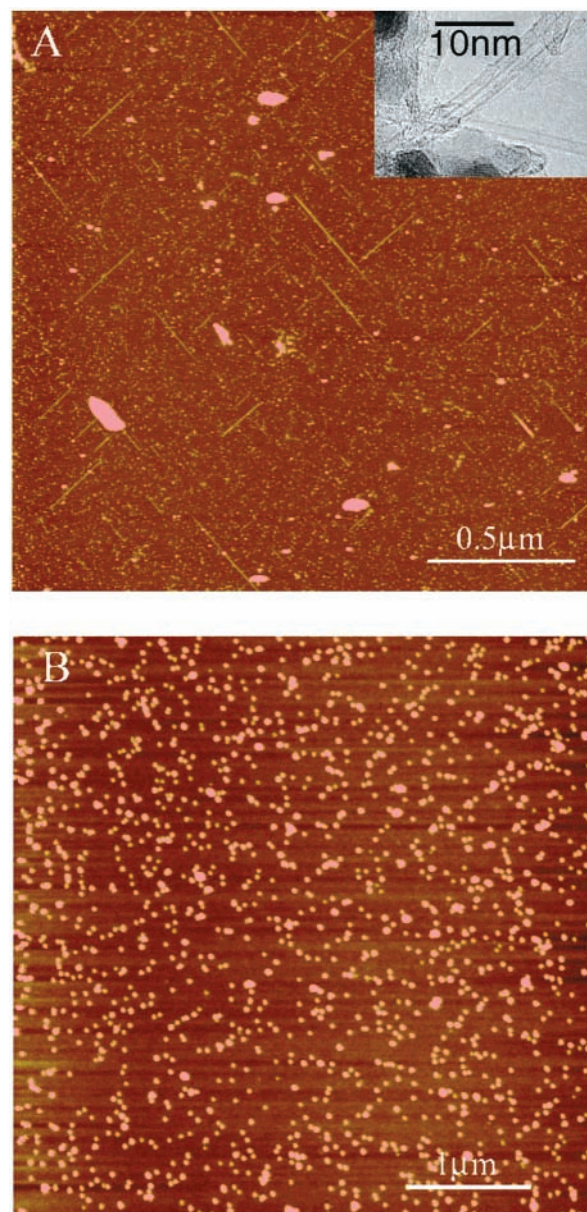
Figure 8. AFM images of the Al 2 O 3 /Si wafers with 3.6 nm (a) and 8.5 nm (b) Fe–Mo nanoparticles on the surface after the CVD process. The insert in (a) shows TEM images of nanotubes grown with 3.6 nm nanoparticles supported on fumed alumina powder under the same growth conditions.
