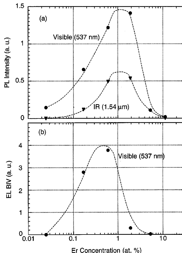
FIG. 2. PL and EL intensity vs Er concentration: (a) visible and IR PL intensity display maxima at \sim 1 at. % Er; (b) visible EL intensity normalized by current flow shows a maximum at \sim 0.5 at. % Er.
