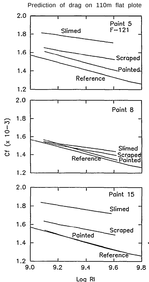
Fig. 4. Prediction of drag on 110 m flat plate.
