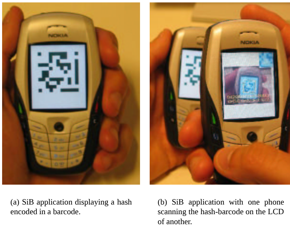
Figure 5: SiB protocol in action.
