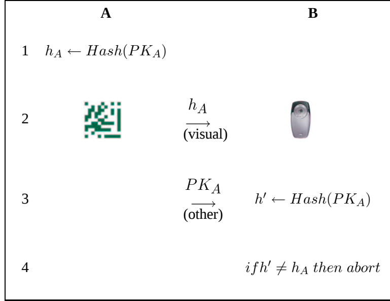
Figure 1: Pre-authentication over the location-limited visual channel. PK_X is X 's public key, which can be either long-term or ephemeral, depending on which standard protocol is selected.
