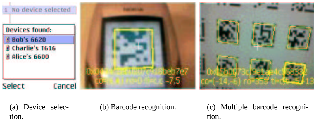
Figure 4: Mobile phone screen shots showing the SiB application in operation. In the first screen shot, the user is being prompted to select a device with which to initiate the SiB protocol. In the second, the user sees the phone at which he is aiming his camera, with status markers indicating successful barcode recognition. The third image is successful recognition of multiple barcodes displayed on an LCD screen.
