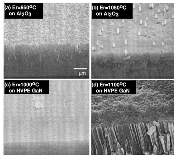
FIG. 2. SEM photos of GaN:Er films on sapphire (a),(b) and HVPE GaN (c),(d).
