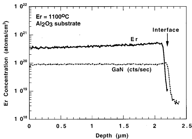
FIG. 5. Er concentration profile for a film grown on sapphire with an Er cell temperature of 1100 °C.
