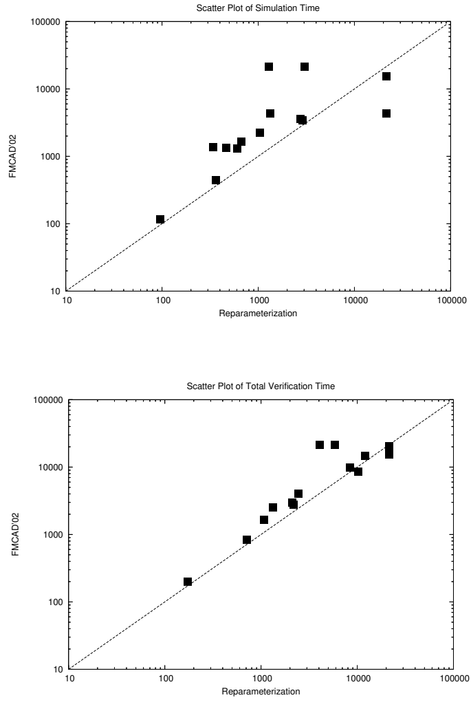
Fig. 1. Scatter plots of simulation time and total time.
