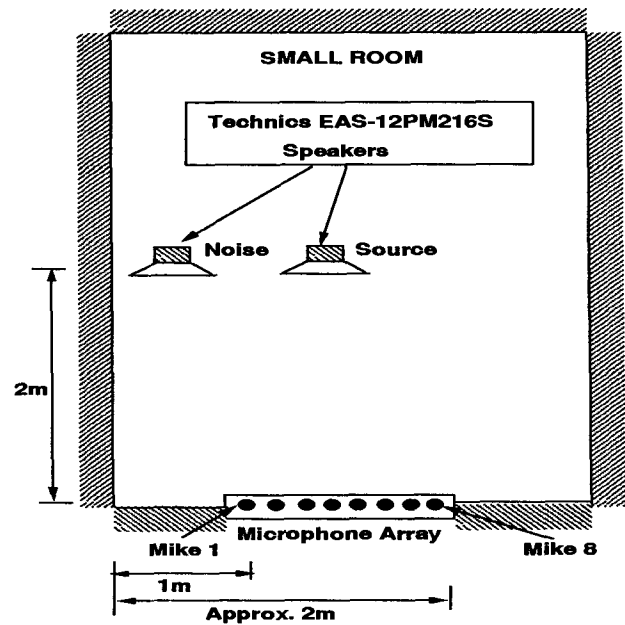
Figure 1: Acoustical Geometry of Array/Sources
