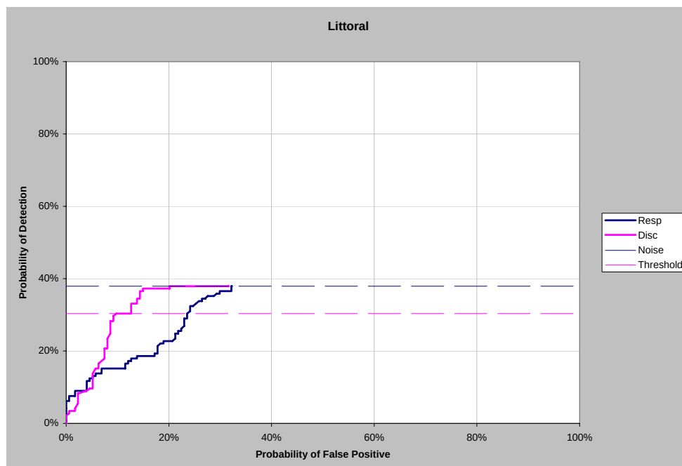
Figure 12. Littoral P_d versus P_{fp} .
