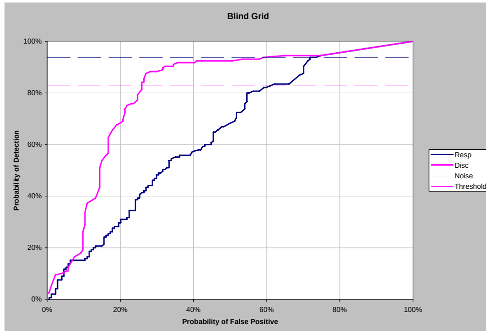
Figure 8. Blind grid P_d versus P_{fp} .
