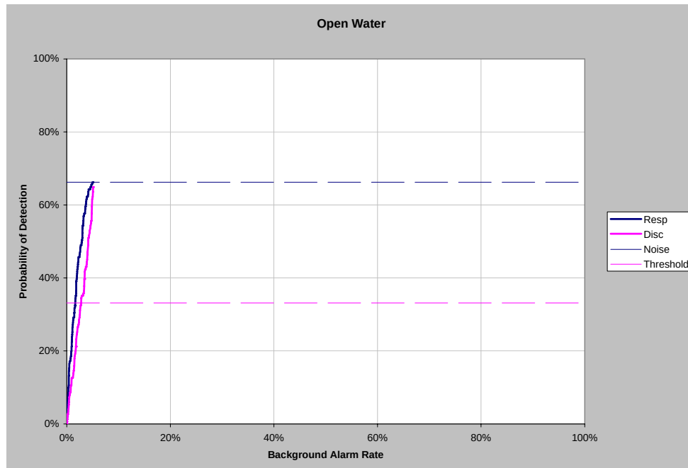
Figure 11. Open water P_d versus BAR.
