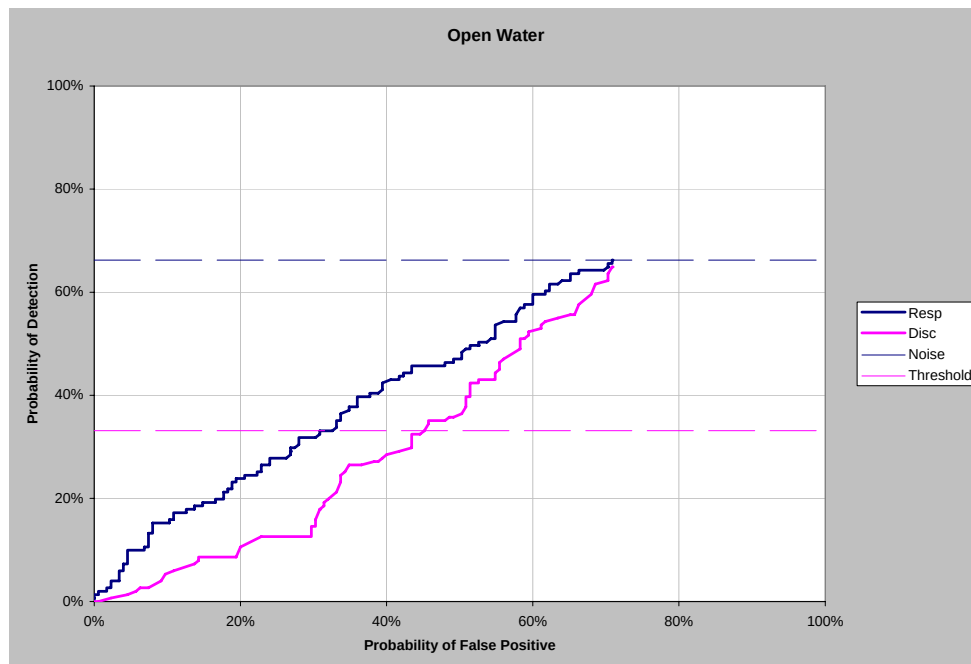
Figure 10. Open water P_d versus P_{fp} .
