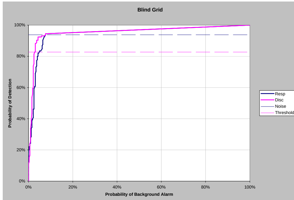
Figure 9. Blind grid P_d versus P_{ba} .
