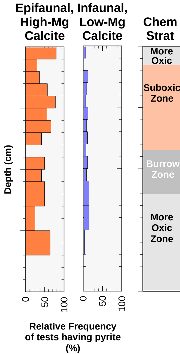
Figure 1. Relative frequency of tests that show heavy boring due to endolithic microorganisms.
