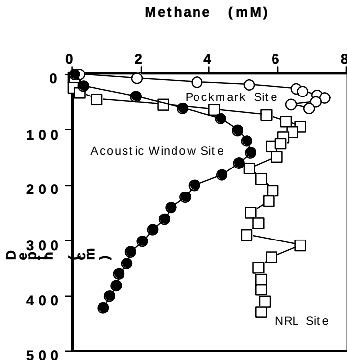
Figure 2. Porewater methane concentration profiles for three Eckemförde Bay sites.
