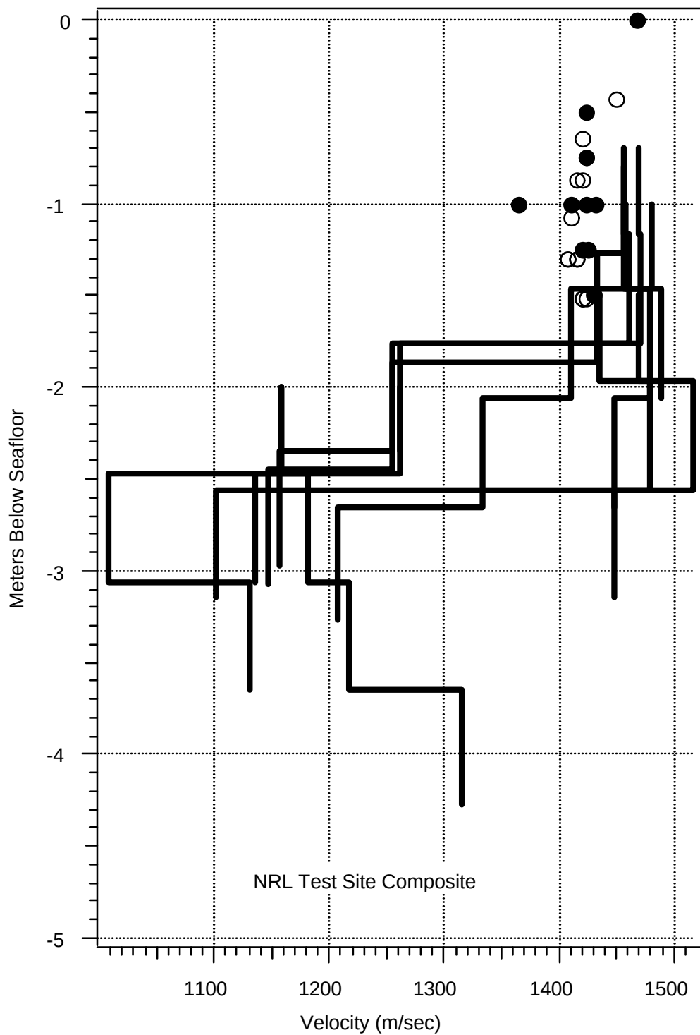
Figure 3. Composite of multiple sites within the NRL test area inside Eckerförde Bay. Circles represent measurements made in situ and on core at frequencies above gas bubble resonance.
