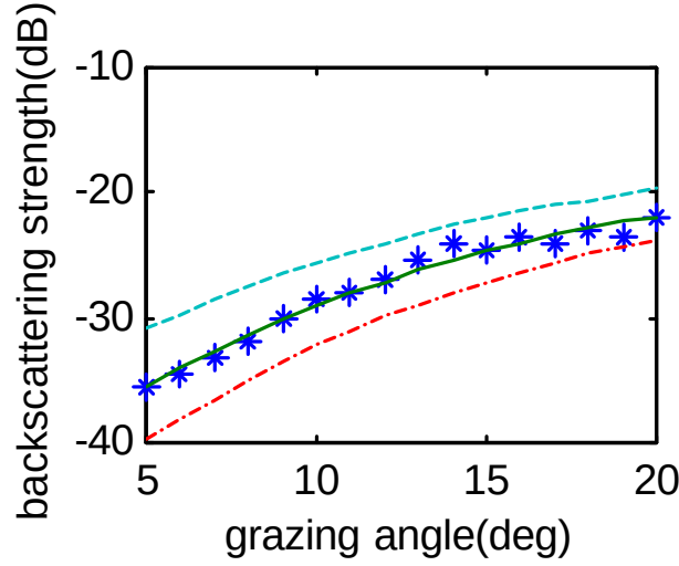
Fig. 2. Model fit to the backscattering strength data of Eckernfoerde Bay. The middle curve is a least-square fit and the other curves are the upper and lower bounds. For details see Ref. 1.
