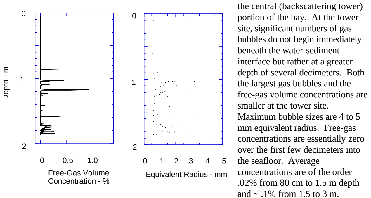
Figure 4 Bubble population data for Core 707-BS-DC (P2)
