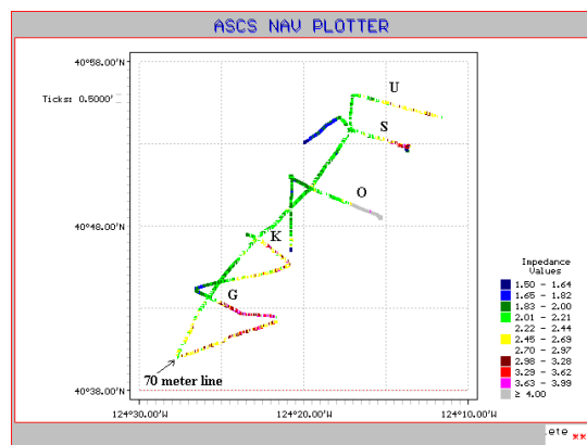
Figure 1. NRL/Acoustic Seafloor Classification System (ASCS) real time trackplot of acoustic impedance obtained using 15 kHz during Leg 1 of R/V WECOMA Cruise W9605B (Eel River). Grays are off scale and result from improper settings and should actually be in red color zone. Reds are coastal sands. Yellow and green colors indicate areas which transition from softer muddy sands to muds (or silts), respectively. Blues are indicative of very soft silts or muds.
