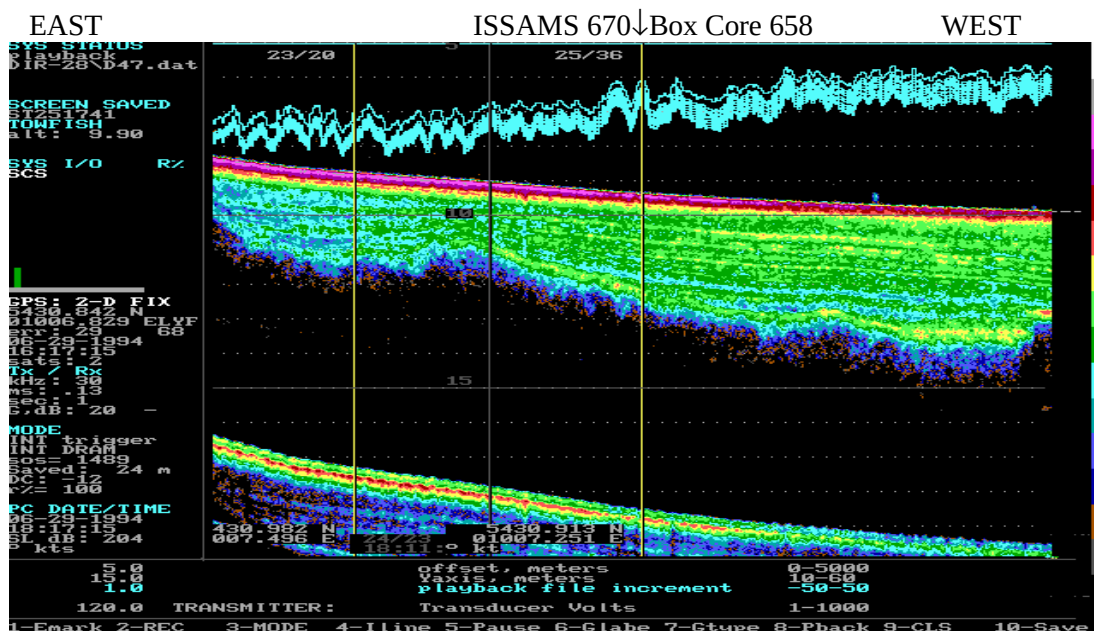
Figure 6a. ASCS 30 kHz seismic record across Line 47 showing the location of Core Site 658 and ISSAMS Site 670 in Eckernfoerder Bay, Germany.
