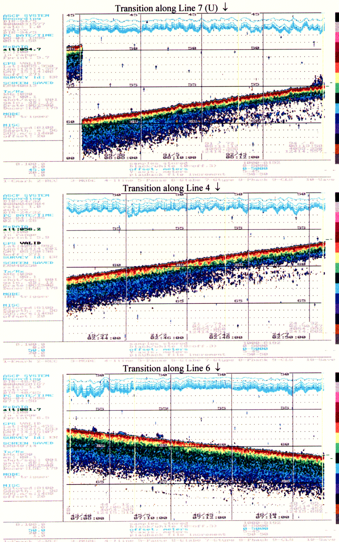
Figure 3. 30-KHz ASCS acoustic imagery along designated lines displaying sediment transitions.
