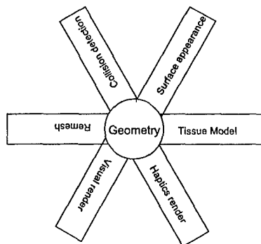
Figure 1. Software Architecture
