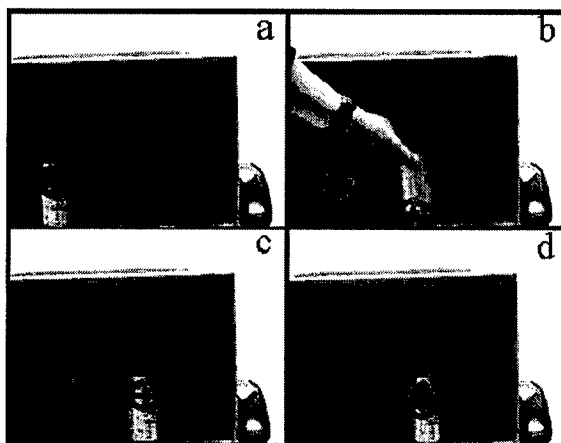
Fig. 7. a) Targeting laser on detected vulnerability (soda can); b) Can is tracked in real-time while being relocated; c) Targeting laser servos to new location; d) Laser now relocated on new target position, ready to fire weapon.
