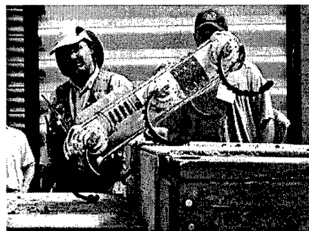
Fig 2. DARPA's RHex prototype employs six dynamically controlled rotating "legs" for enhanced mobility in rough terrain.
