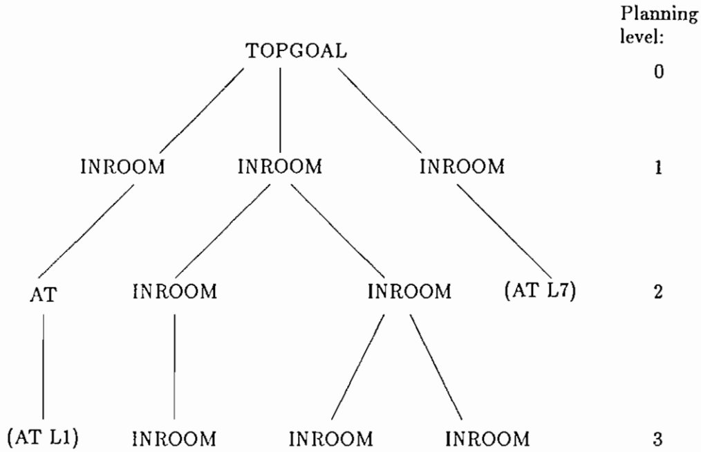
Figure 1: Hierarchical Plan in Robot Domain
