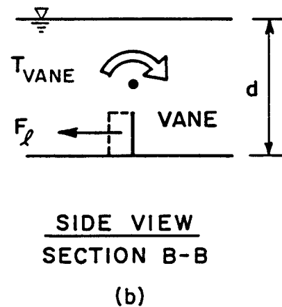
Figure 27 - Definition Sketch for the Calculation of the Torque Produced by (a) the Flow and (b) a Submerged Vane
