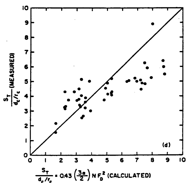
Figure 3 - Comparison of Transverse Bed Slopes Measured by Zimmermann and Kennedy (1978) with Slopes Computed by the Models of (a) van Bendegom (1947); (b) Engelund (1974); (c) Kikkawa, Ikeda, and Kitagawa (1976); (d) Zimmermann and Kennedy (1978) or Falcon (1979); and (e) Odgaard (1981)
