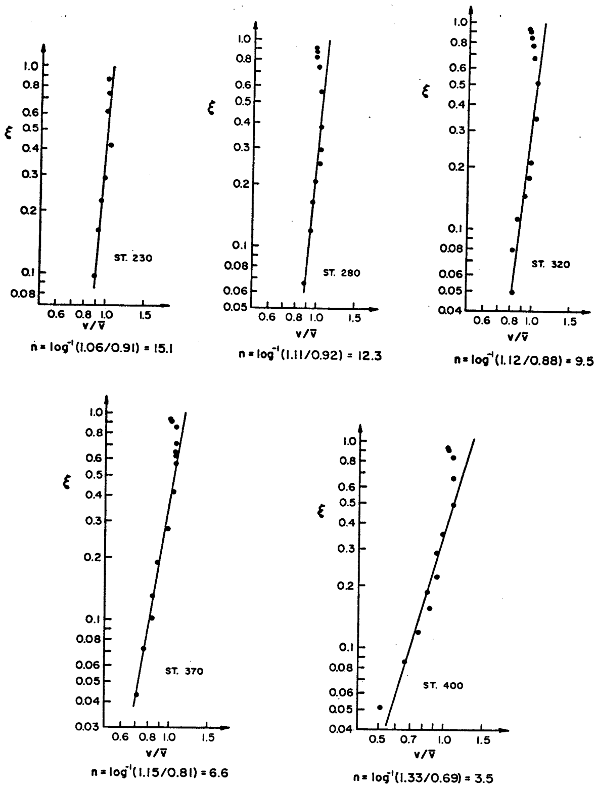
Figure A-8 - Vertical Velocity Distributions in Cross Section No. 4 at High Flow, 24,900 Cubic Feet Per Second
