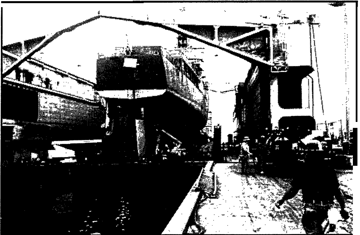
Figure 2.1.b: Vessel drydocked at South West Marine for minor repairs. Notice the flying bridge that allows accessibility to both of the wing walls
