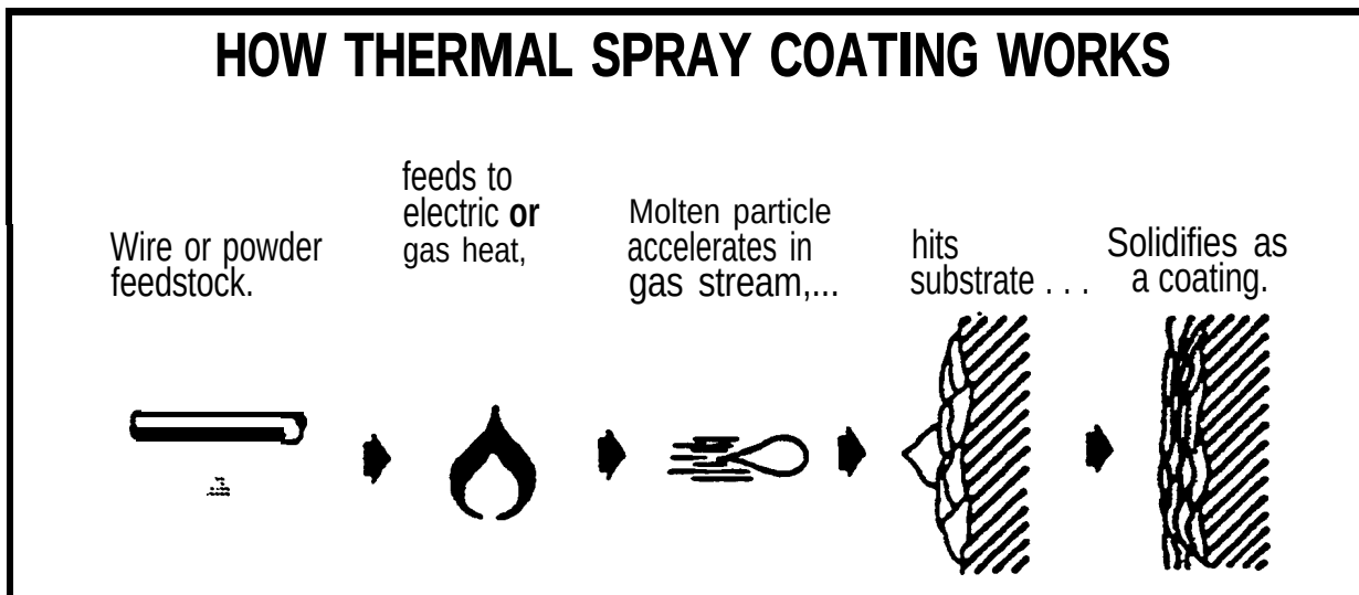
Figure 4.4: Illustration of how thermal coating systems work
