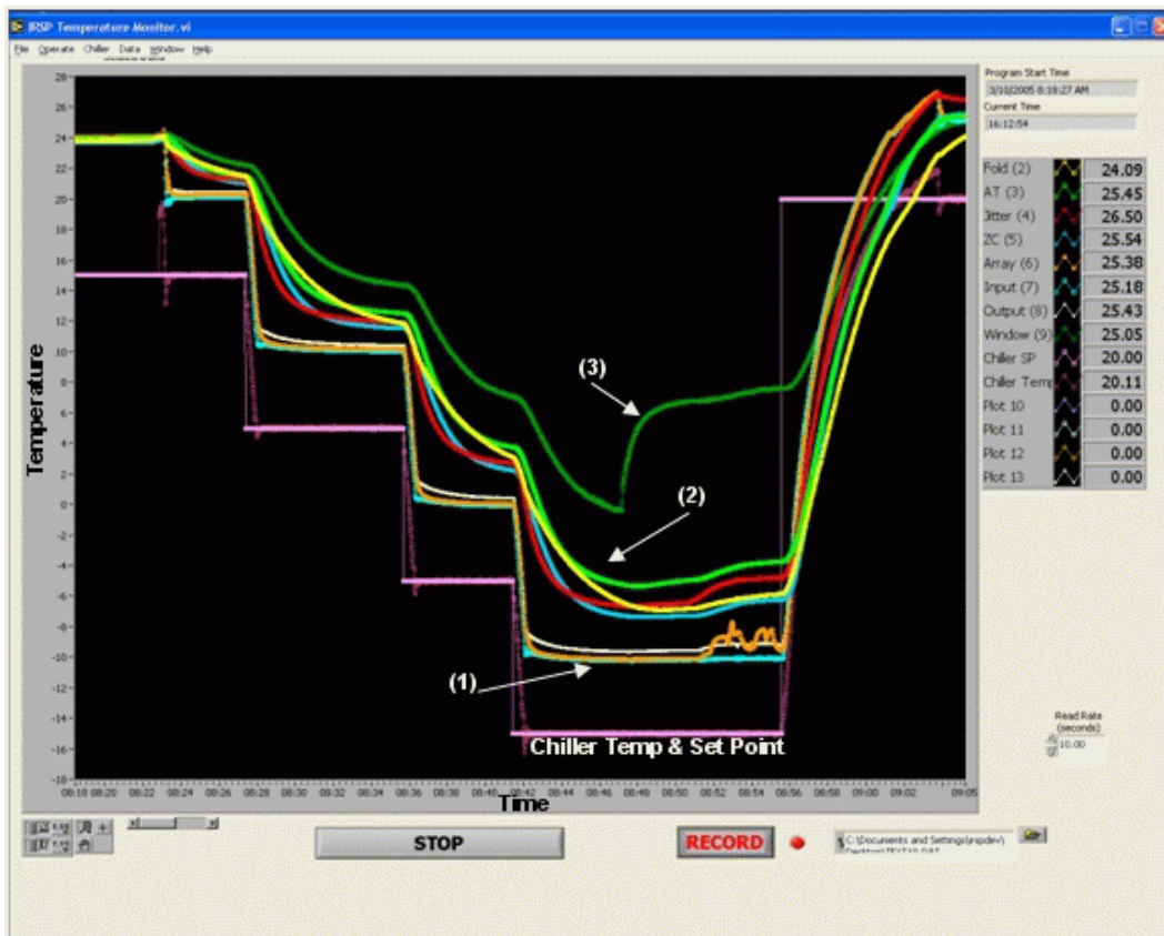
Figure 6: Cool-down Testing
