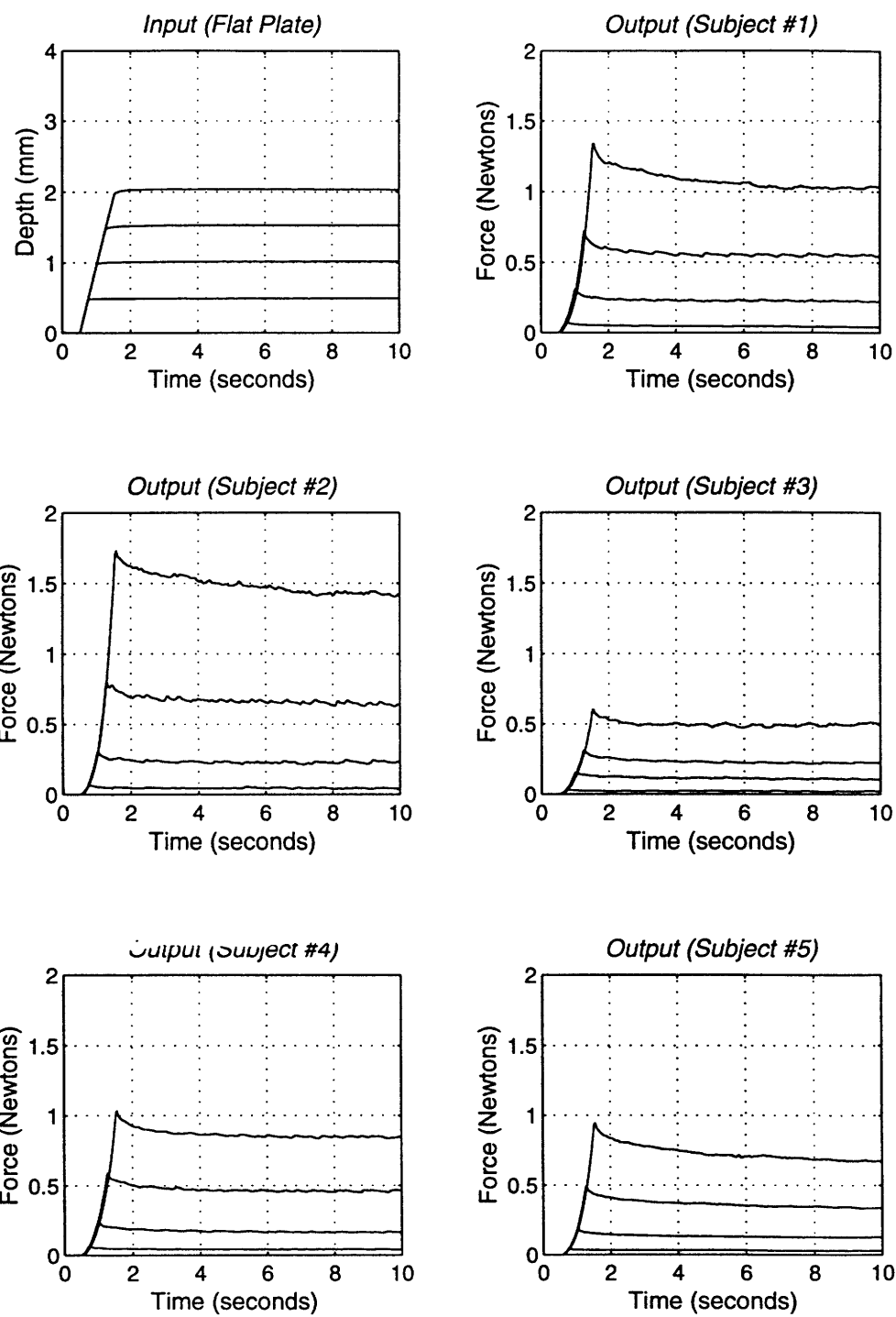
Figure 6-5 (c): Ramp/hold results with flat plate indenter for all depths and ramp velocity of 2 mm/sec.
