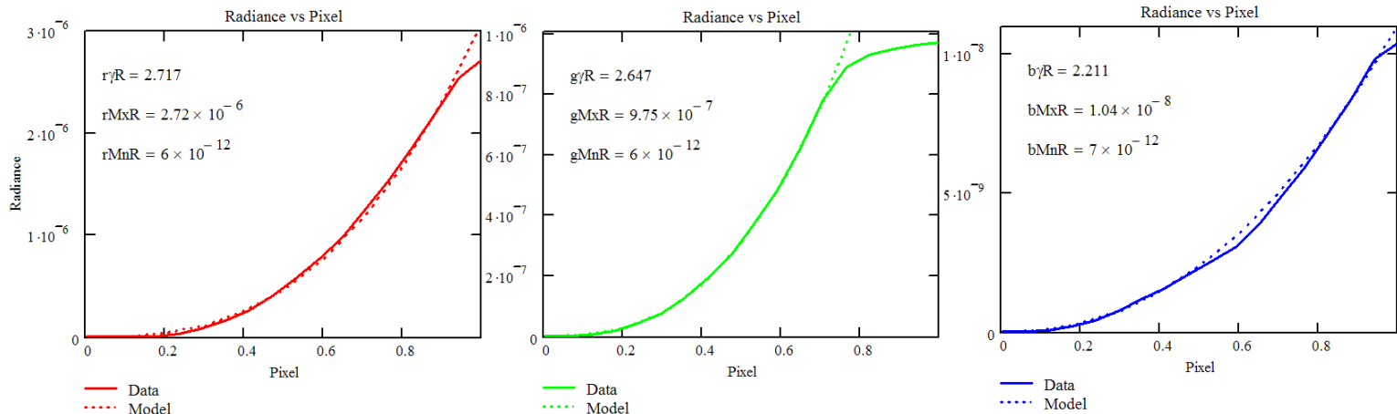
Figure 30 Barco RetroGraphics 801s Radiance Transfer Function Curves
