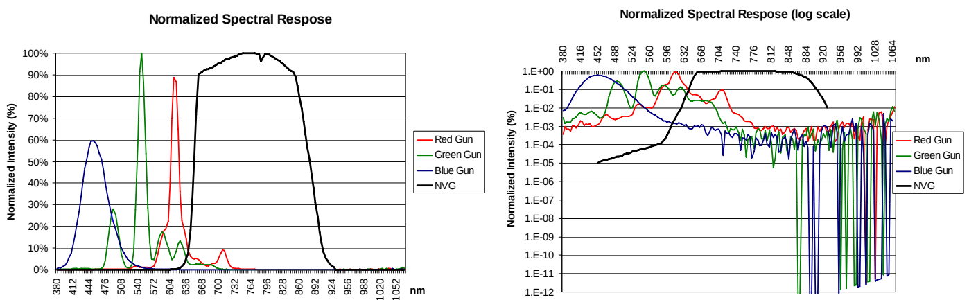
Figure 6 Barco RetroGraphics 801s CRTs Normalized Spectral Response
