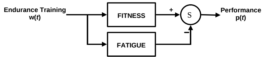
Figure 4. Simple 2-component systems model of training and performance. Diagram shows how training input w(t) affects both fitness and fatigue. The summer (S) combines these responses, fitness positively and fatigue negatively, into a single performance output p(t) (Morton et al. 1990).
