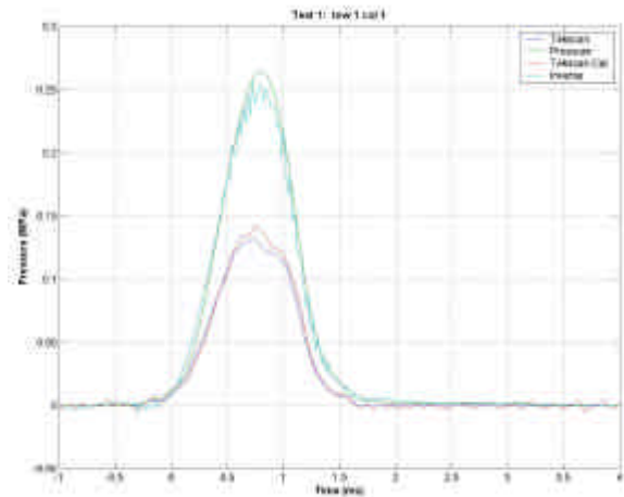
Comparison of pressure measured from one cell of the Bulls Eye Sensor compared to that calculated from a force gauge
