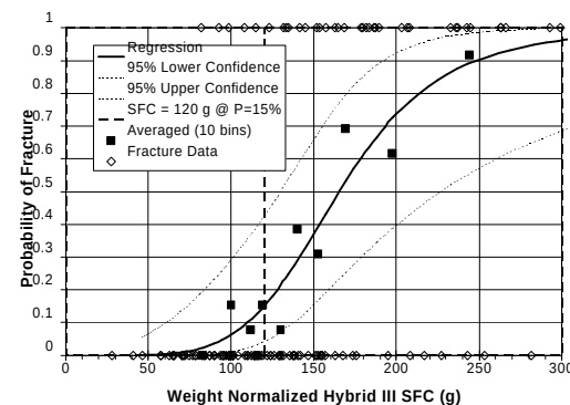
Logistic regression of SFC to skull fracture
