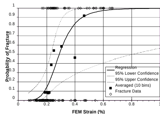
Logistic regression of calculated strain to skull fracture
