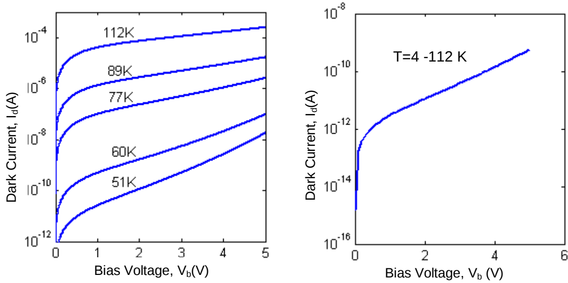
Figure 13: (a) Theoretical curves for the same structure as figure 12 calculated from equation 1. (b) Similar curves with the assumption of conserved lateral momentum.
