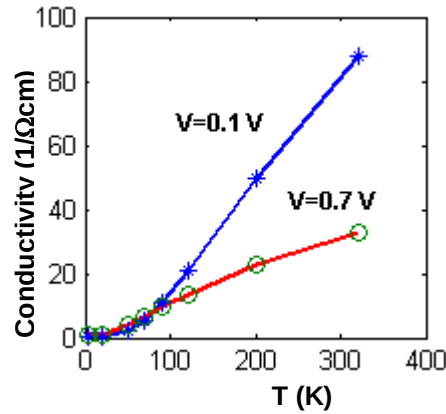
Figure 10: Effective conductivity vs. temperature for the structure of figure 5 assuming non-conserved lateral momentum.
