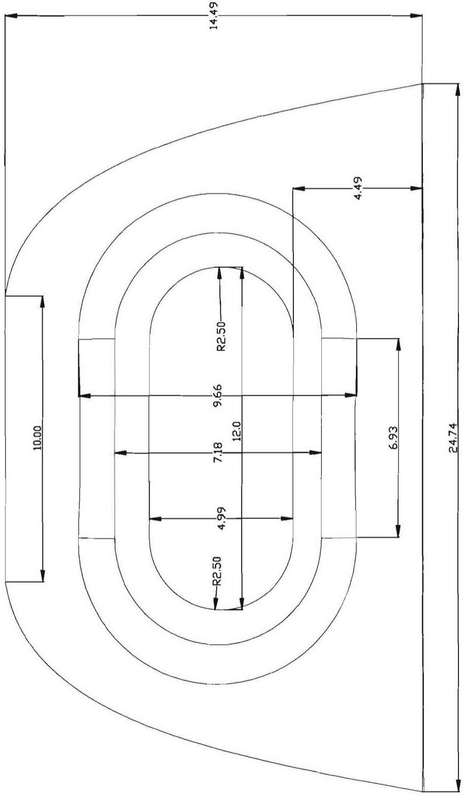
PIN INSERT 1 BOTTOM VIEW
