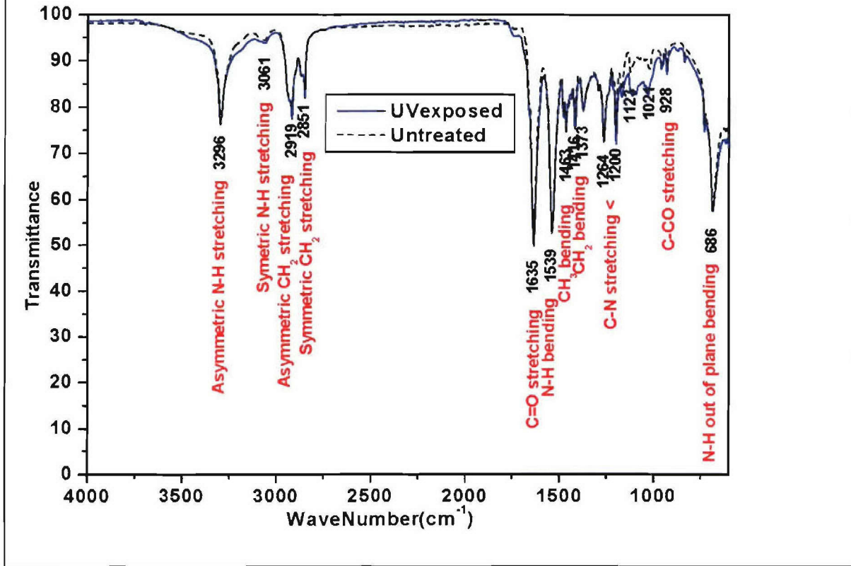
Figure 5-10: UV Radiation Exposed Sample FTIR Spectroscopy Results
