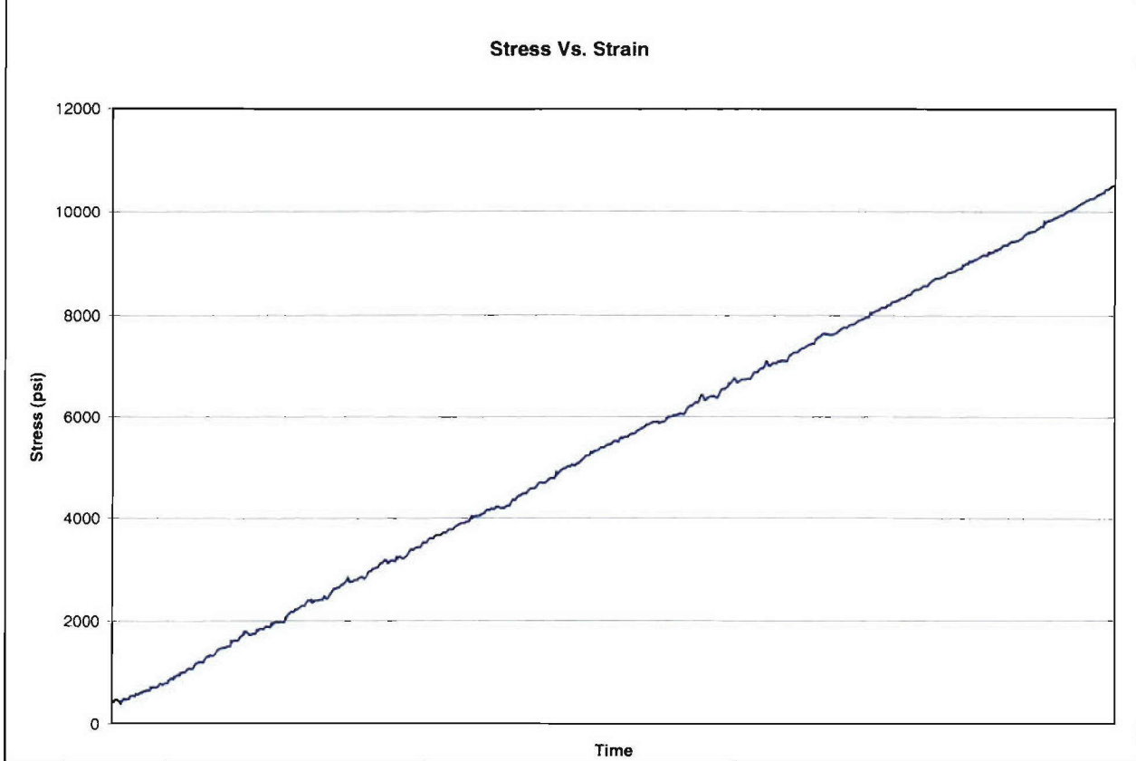
Figure 7-18: Cylindrical Load to Failure Stress versus Time
