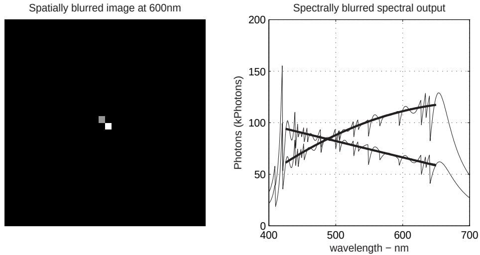
Figure 5.18: Spatially and spectrally reconstructed image and spectral output of a 0.25su radius 10000K and a 5su radius 5000K binary star at 25 light years in the visible. The thin solid line is the reconstruction and the thick line is a least-squares polynomial fit to the reconstruction to smooth out some discontinuities. The true spectra is shown in a dashed line and cannot be seen since it is coincident with the MMSE fit to the reconstruction.
