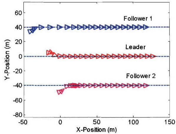
Figure 3: Vehicle Trajectories
