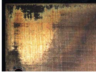
Figure 7: MIL-PRF-21260 15W40 (Copper - 3b corrosion at 135°C)
