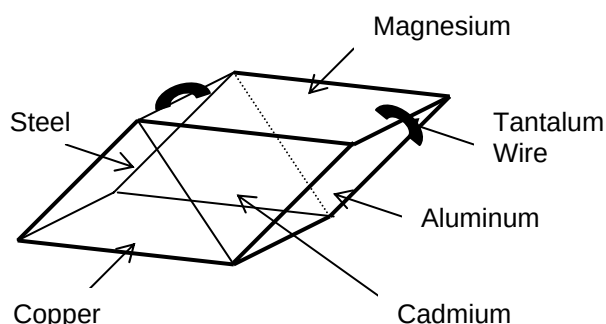
Figure 5: Arrangement of metal test specimens 17 .
