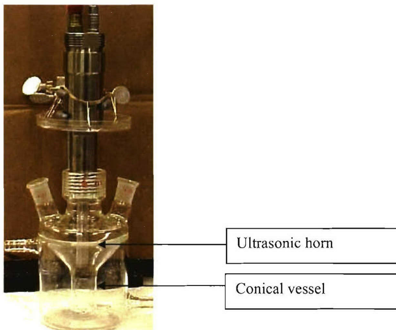
Figure 1. Conical vessel and HPU transducer used for beaker-scale experiments on bacteria and zooplankton.
