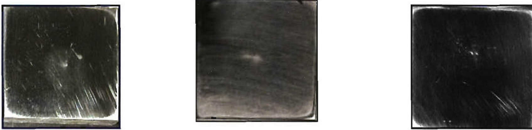
Figure 18. Photographs of test coupons following 12 hours exposure to cavitation: alloy 686 at separation distances of 0.01 inches (left), 0.03 inches (center), and 1 inch titanium (right).
