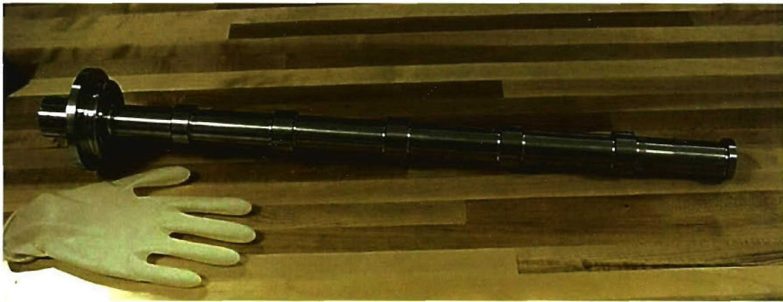
Figure 5. Ultrasonic Treatment Cascade Horn.
