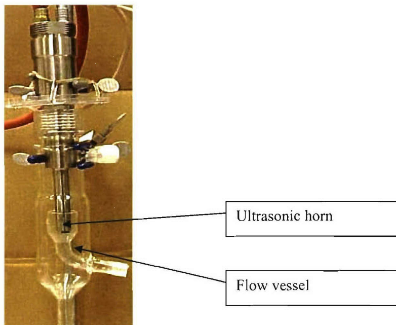
Figure 2. Flow vessel and HPU transducer used for bench-scale experiments on zooplankton.
