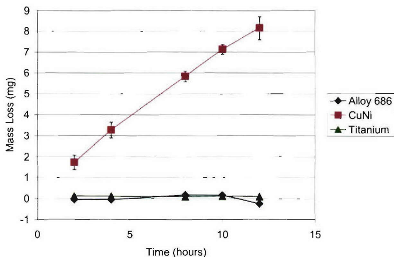
Figure 15. Cavitation erosion results for alloy 686, CP titanium, and CuNi at a various flow rates and pressures (separation distance 0.03-in.) The error bars represent the standard deviation of the mean of three trials and in most cases are smaller than the size of the datapoint.
