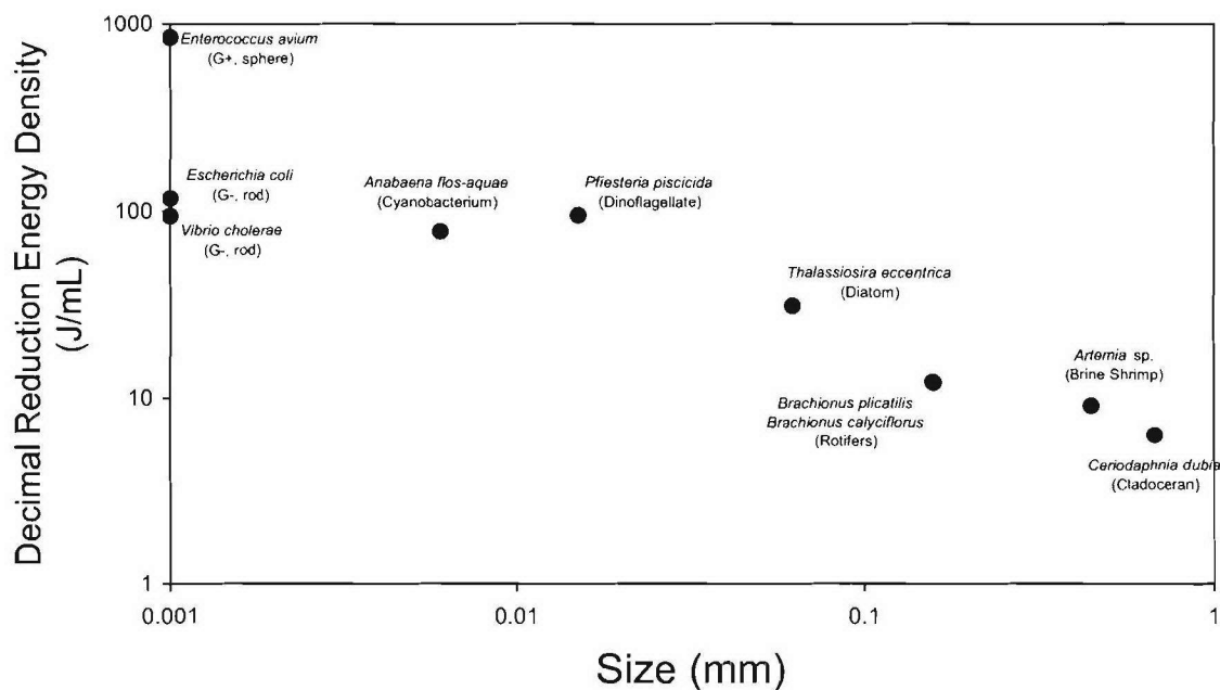
Figure 10. Plot of decimal reduction energy density versus organism size for the various organisms tested.
