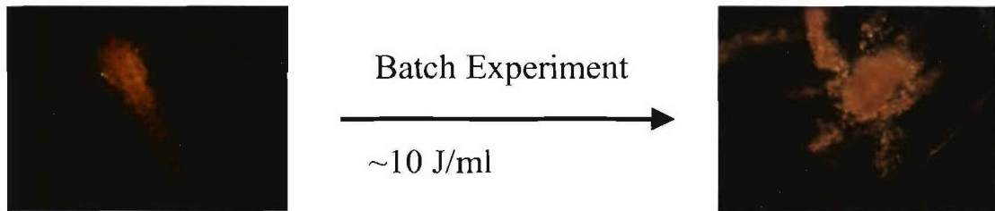
Figure 9. Micrographs of Artemia , before (left) and after (right) exposure to HPU in a batch treatment system.
